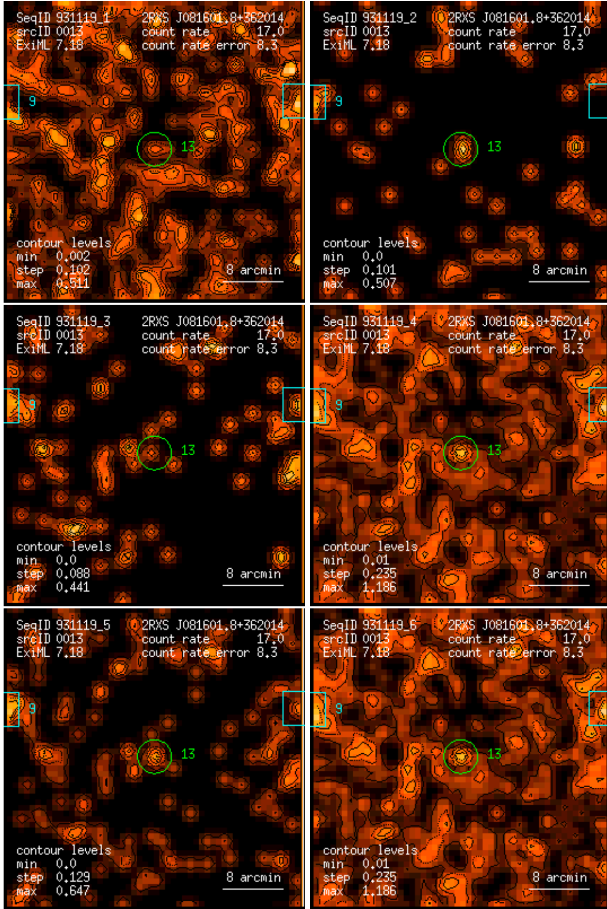
Figure 13: RASS 931119: detection 0013: band rate images, Gaussian filter: (1) PSPC channels 11 – 41, (2) 52 – 90, (3) 91 – 201, (4) 11 – 235, (5) 52 – 201, (6) 11 – 201. Broad band rates in counts/ks. Band rate contour levels in counts/ks/arcmin 2 .
