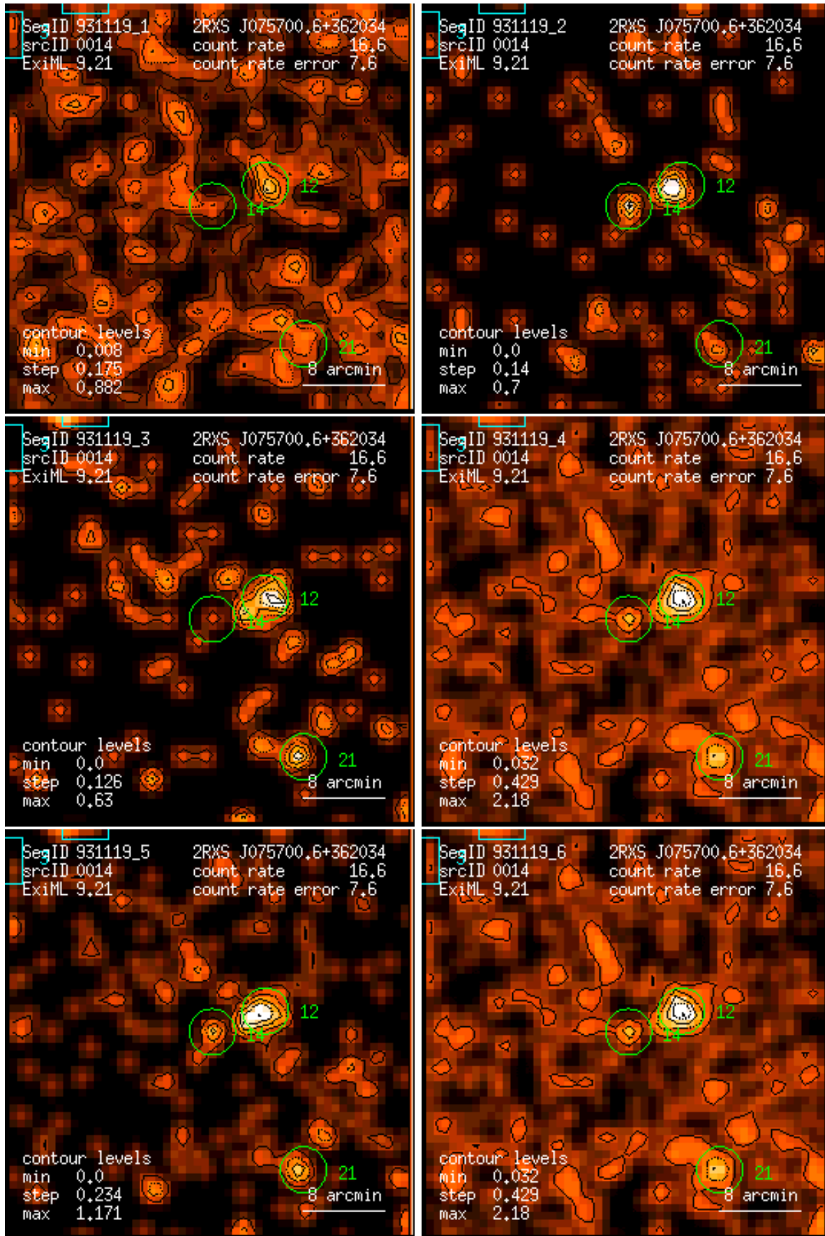
Figure 14: RASS 931119: detection 0014: band rate images, Gaussian filter: (1) PSPC channels 11 – 41, (2) 52 – 90, (3) 91 – 201, (4) 11 – 235, (5) 52 – 201, (6) 11 – 201. Broad band rates in counts/ks. Band rate contour levels in counts/ks/arcmin 2 .
