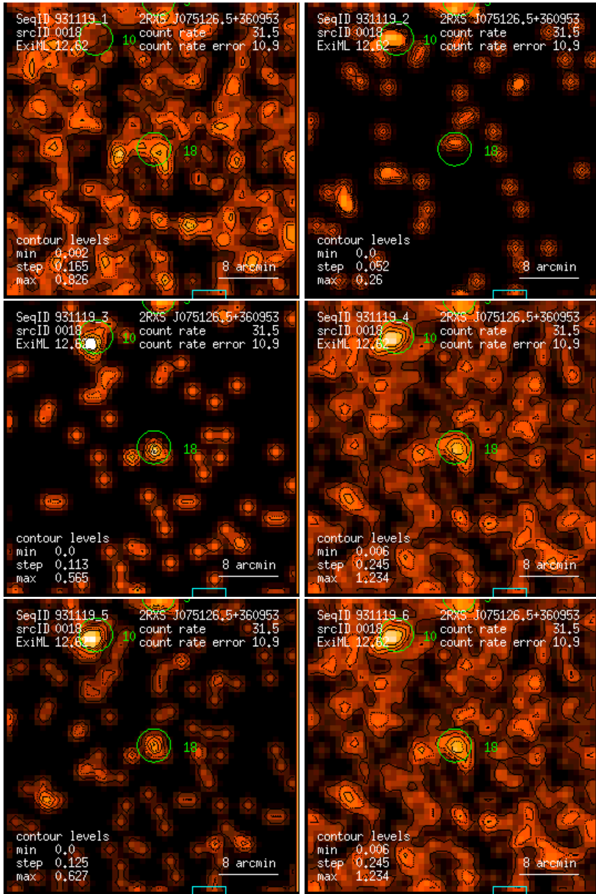
Figure 18: RASS 931119: detection 0018: band rate images, Gaussian filter: (1) PSPC channels 11 – 41, (2) 52 – 90, (3) 91 – 201, (4) 11 – 235, (5) 52 – 201, (6) 11 – 201. Broad band rates in counts/ks. Band rate contour levels in counts/ks/arcmin 2 .
