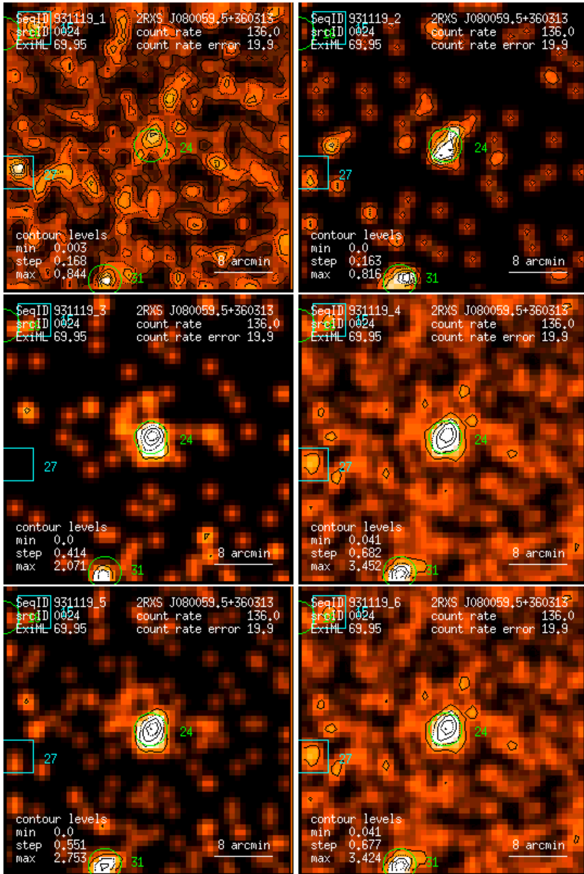
Figure 24: RASS 931119: detection 0024: band rate images, Gaussian filter: (1) PSPC channels 11 – 41, (2) 52 – 90, (3) 91 – 201, (4) 11 – 235, (5) 52 – 201, (6) 11 – 201. Broad band rates in counts/ks. Band rate contour levels in counts/ks/arcmin 2 .
