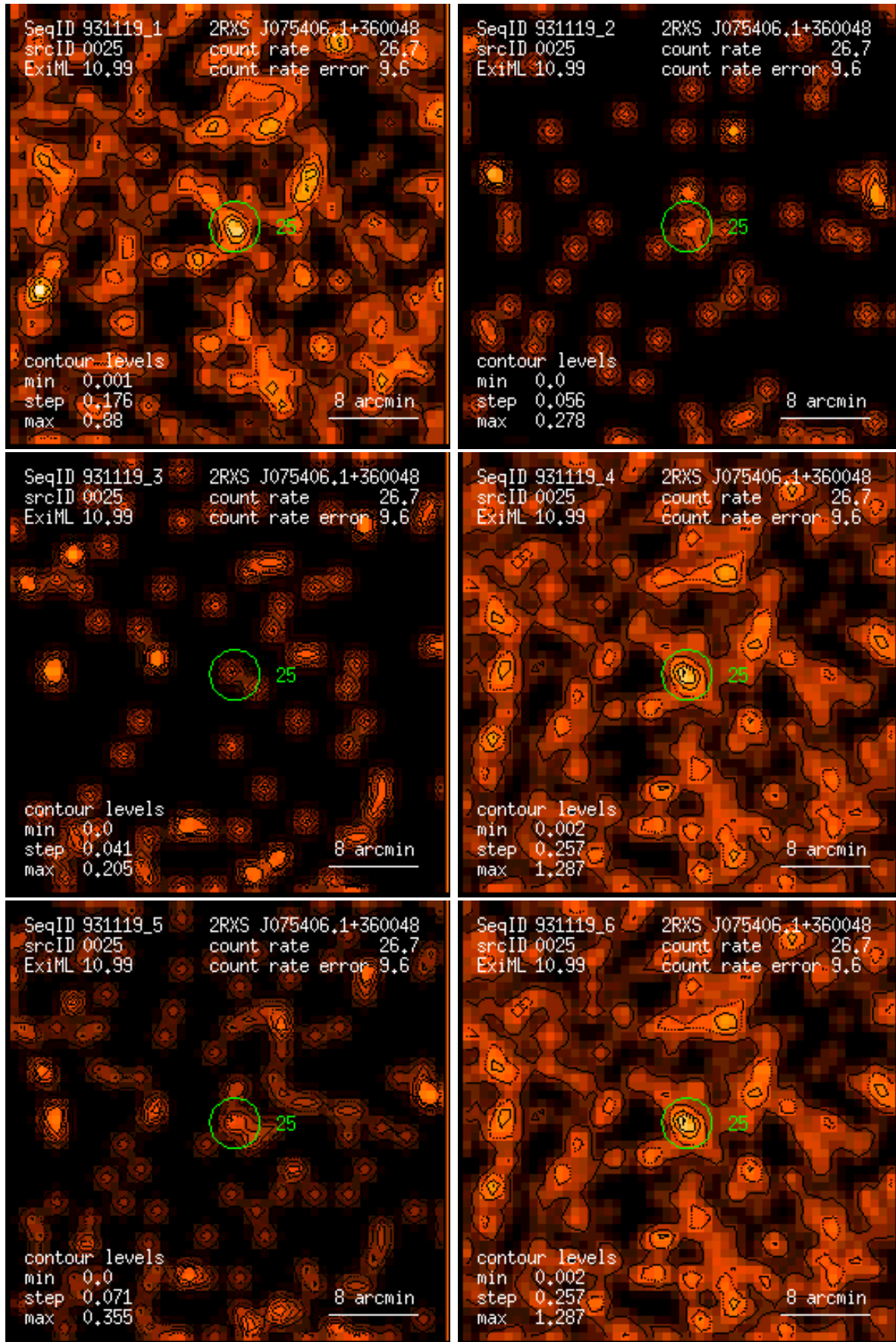
Figure 25: RASS 931119: detection 0025: band rate images, Gaussian filter: (1) PSPC channels 11 – 41, (2) 52 – 90, (3) 91 – 201, (4) 11 – 235, (5) 52 – 201, (6) 11 – 201. Broad band rates in counts/ks. Band rate contour levels in counts/ks/arcmin 2 .
