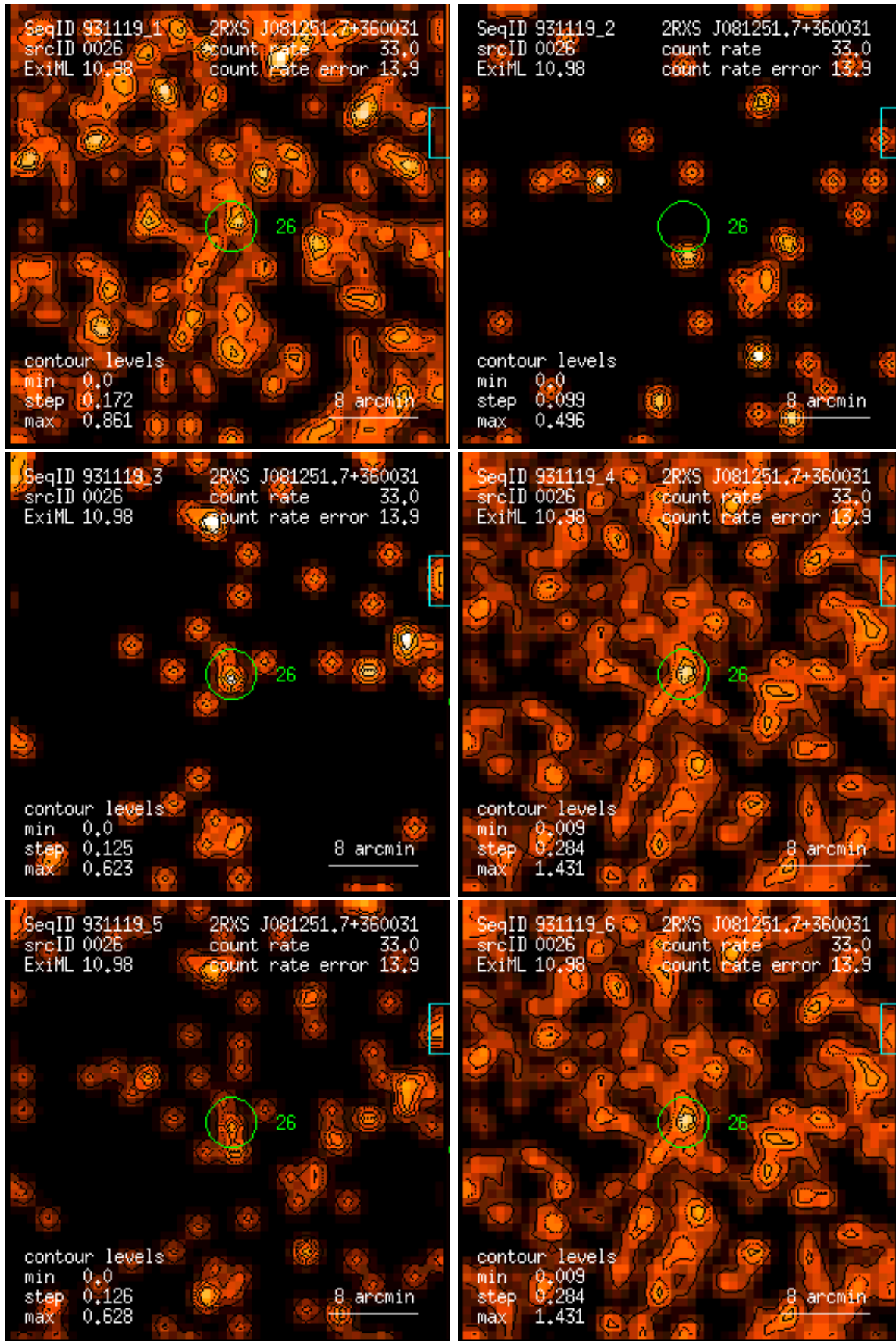
Figure 26: RASS 931119: detection 0026: band rate images, Gaussian filter: (1) PSPC channels 11 – 41, (2) 52 – 90, (3) 91 – 201, (4) 11 – 235, (5) 52 – 201, (6) 11 – 201. Broad band rates in counts/ks. Band rate contour levels in counts/ks/arcmin 2 .
