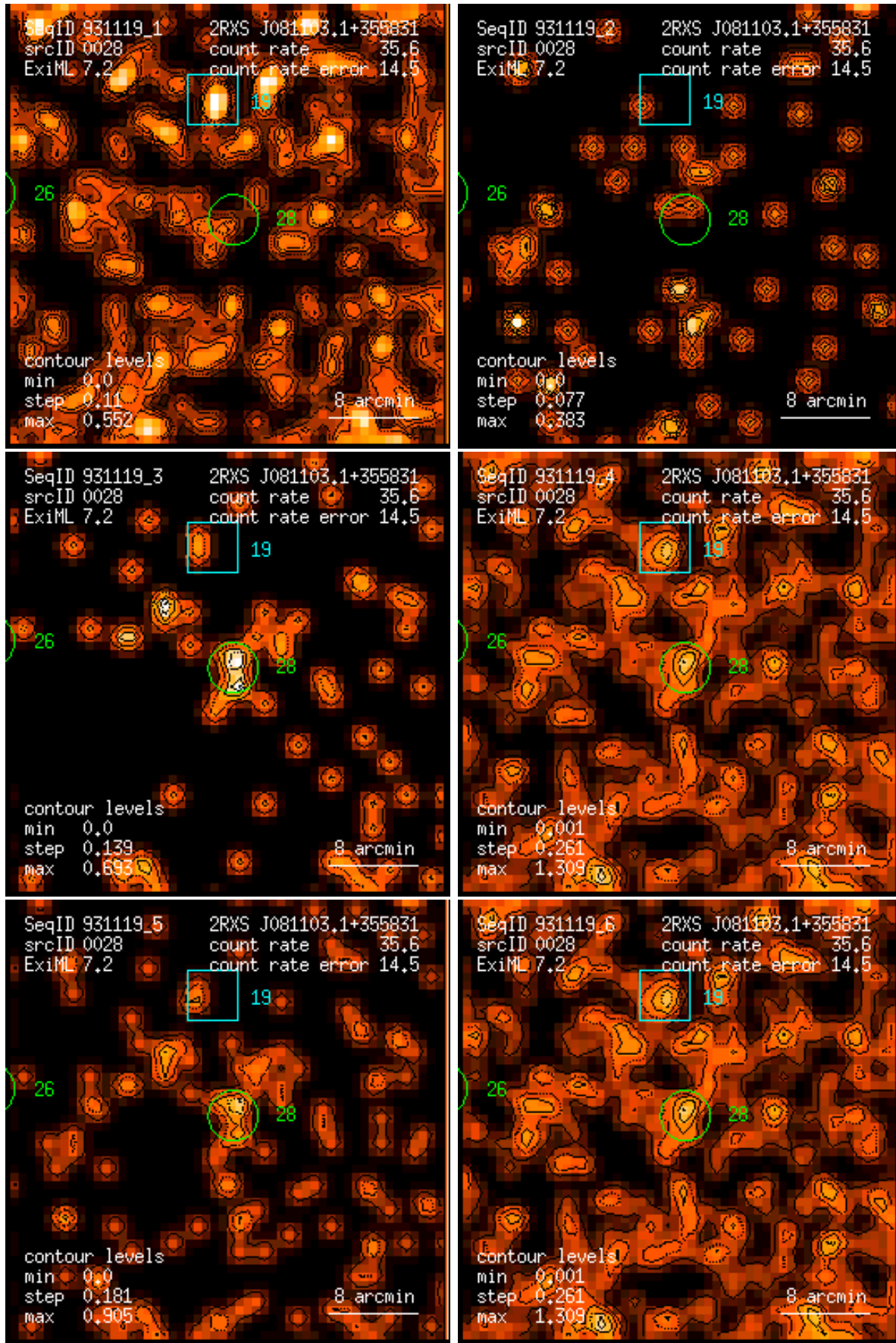
Figure 28: RASS 931119: detection 0028: band rate images, Gaussian filter: (1) PSPC channels 11 – 41, (2) 52 – 90, (3) 91 – 201, (4) 11 – 235, (5) 52 – 201, (6) 11 – 201. Broad band rates in counts/ks. Band rate contour levels in counts/ks/arcmin 2 .
