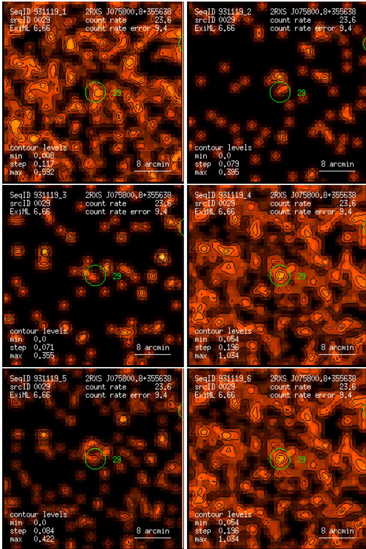
Figure 29: RASS 931119: detection 0029: band rate images, Gaussian filter: (1) PSPC channels 11 – 41, (2) 52 – 90, (3) 91 – 201, (4) 11 – 235, (5) 52 – 201, (6) 11 – 201. Broad band rates in counts/ks. Band rate contour levels in counts/ks/arcmin 2 .
