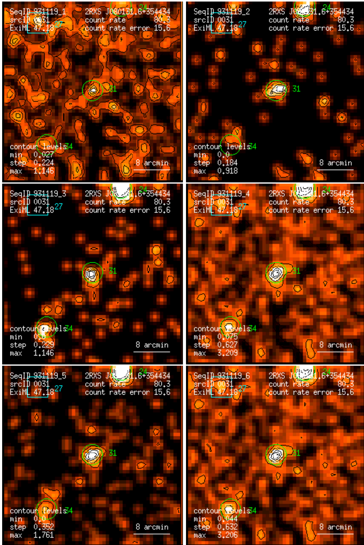
Figure 31: RASS 931119: detection 0031: band rate images, Gaussian filter: (1) PSPC channels 11 – 41, (2) 52 – 90, (3) 91 – 201, (4) 11 – 235, (5) 52 – 201, (6) 11 – 201. Broad band rates in counts/ks. Band rate contour levels in counts/ks/arcmin 2 .
