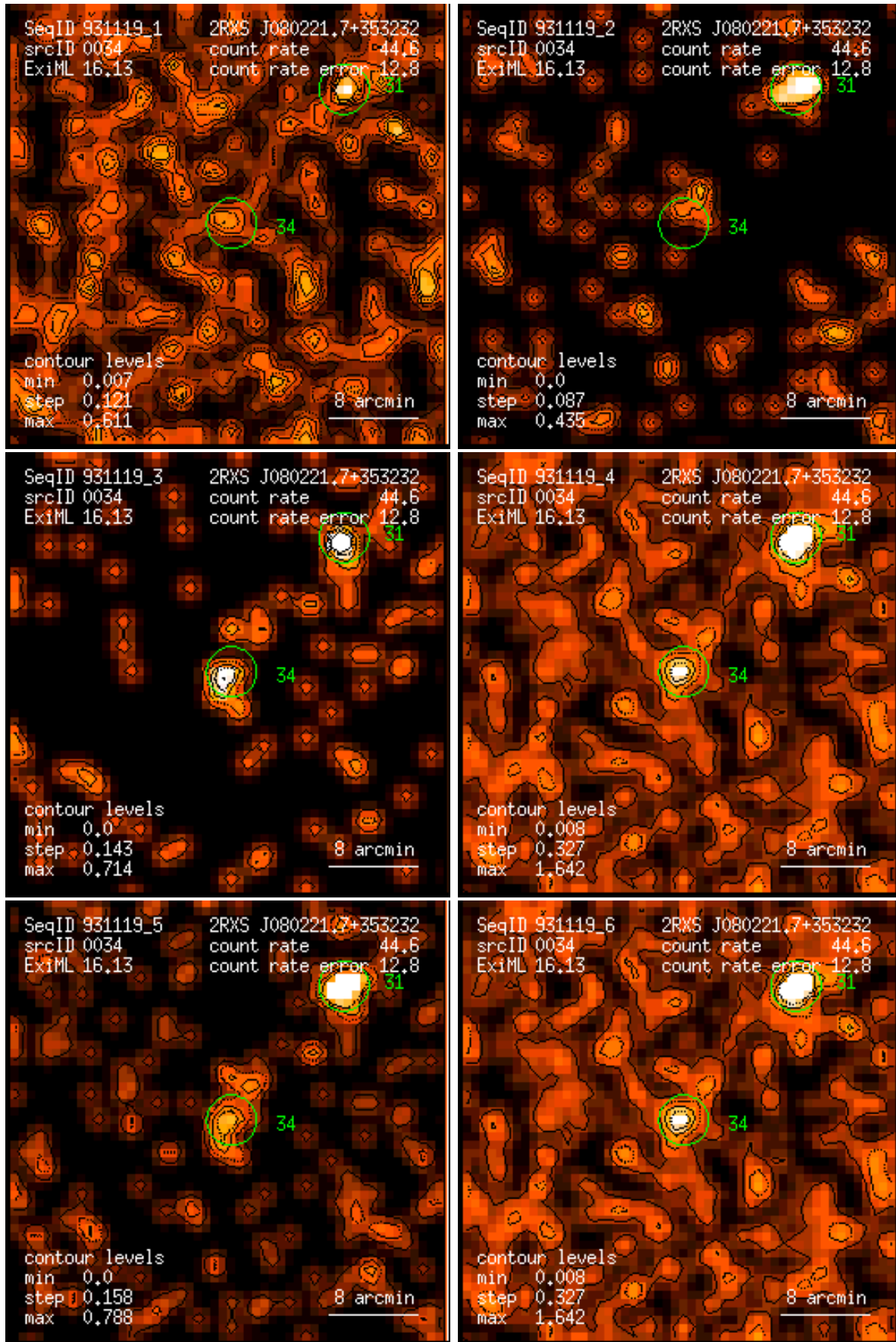
Figure 34: RASS 931119: detection 0034: band rate images, Gaussian filter: (1) PSPC channels 11 – 41, (2) 52 – 90, (3) 91 – 201, (4) 11 – 235, (5) 52 – 201, (6) 11 – 201. Broad band rates in counts/ks. Band rate contour levels in counts/ks/arcmin 2 .
