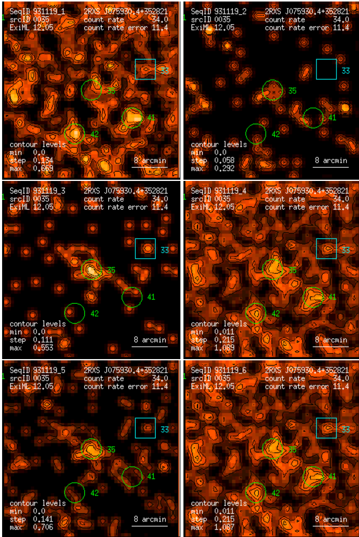
Figure 35: RASS 931119: detection 0035: band rate images, Gaussian filter: (1) PSPC channels 11 – 41, (2) 52 – 90, (3) 91 – 201, (4) 11 – 235, (5) 52 – 201, (6) 11 – 201. Broad band rates in counts/ks. Band rate contour levels in counts/ks/arcmin 2 .
