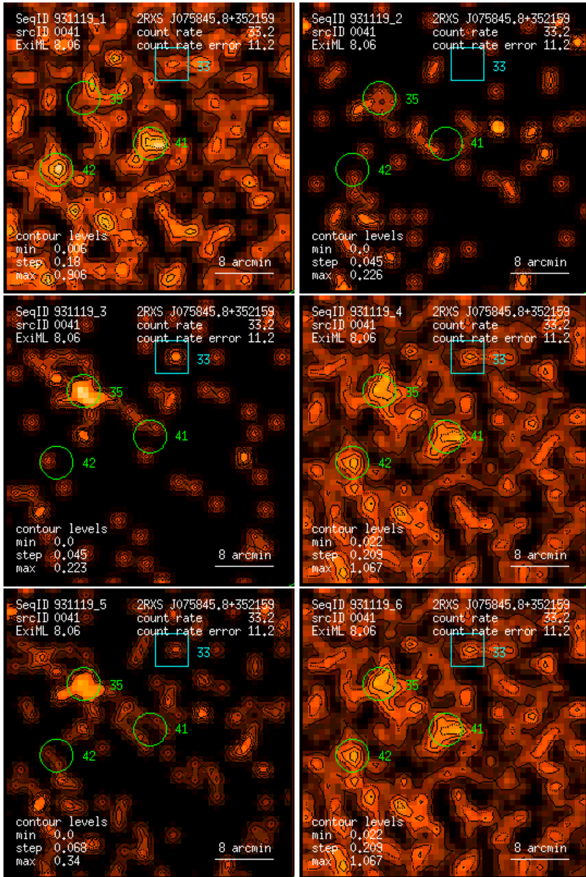
Figure 41: RASS 931119: detection 0041: band rate images, Gaussian filter: (1) PSPC channels 11 – 41, (2) 52 – 90, (3) 91 – 201, (4) 11 – 235, (5) 52 – 201, (6) 11 – 201. Broad band rates in counts/ks. Band rate contour levels in counts/ks/arcmin 2 .
