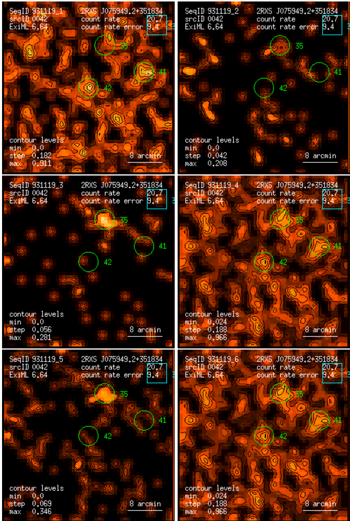
Figure 42: RASS 931119: detection 0042: band rate images, Gaussian filter: (1) PSPPC channels 11 – 41, (2) 52 – 90, (3) 91 – 201, (4) 11 – 235, (5) 52 – 201, (6) 11 – 201. Broad band rates in counts/ks. Band rate contour levels in counts/ks/arcmin 2 .
