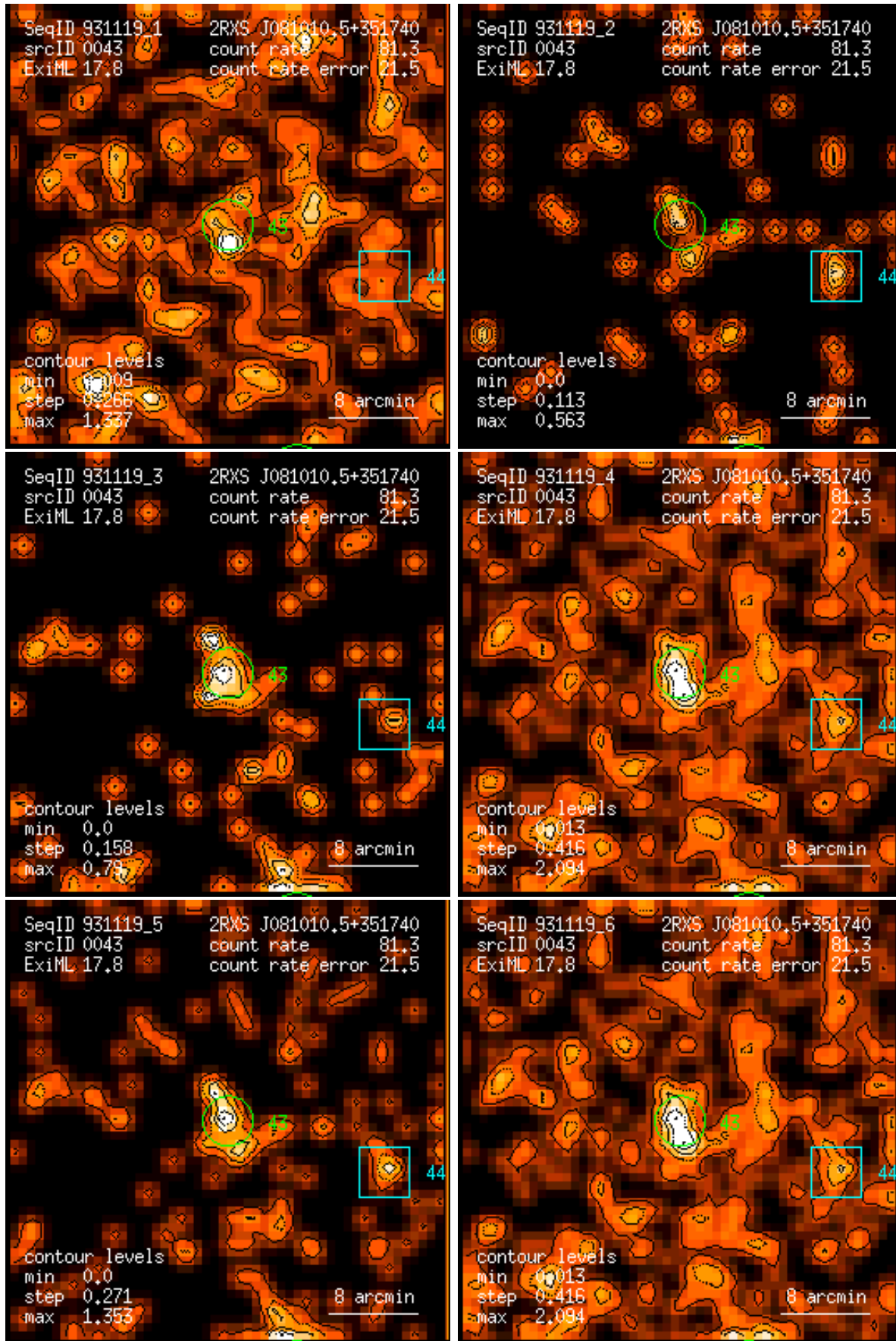
Figure 43: RASS 931119: detection 0043: band rate images, Gaussian filter: (1) PSPC channels 11 – 41, (2) 52 – 90, (3) 91 – 201, (4) 11 – 235, (5) 52 – 201, (6) 11 – 201. Broad band rates in counts/ks. Band rate contour levels in counts/ks/arcmin 2 .
