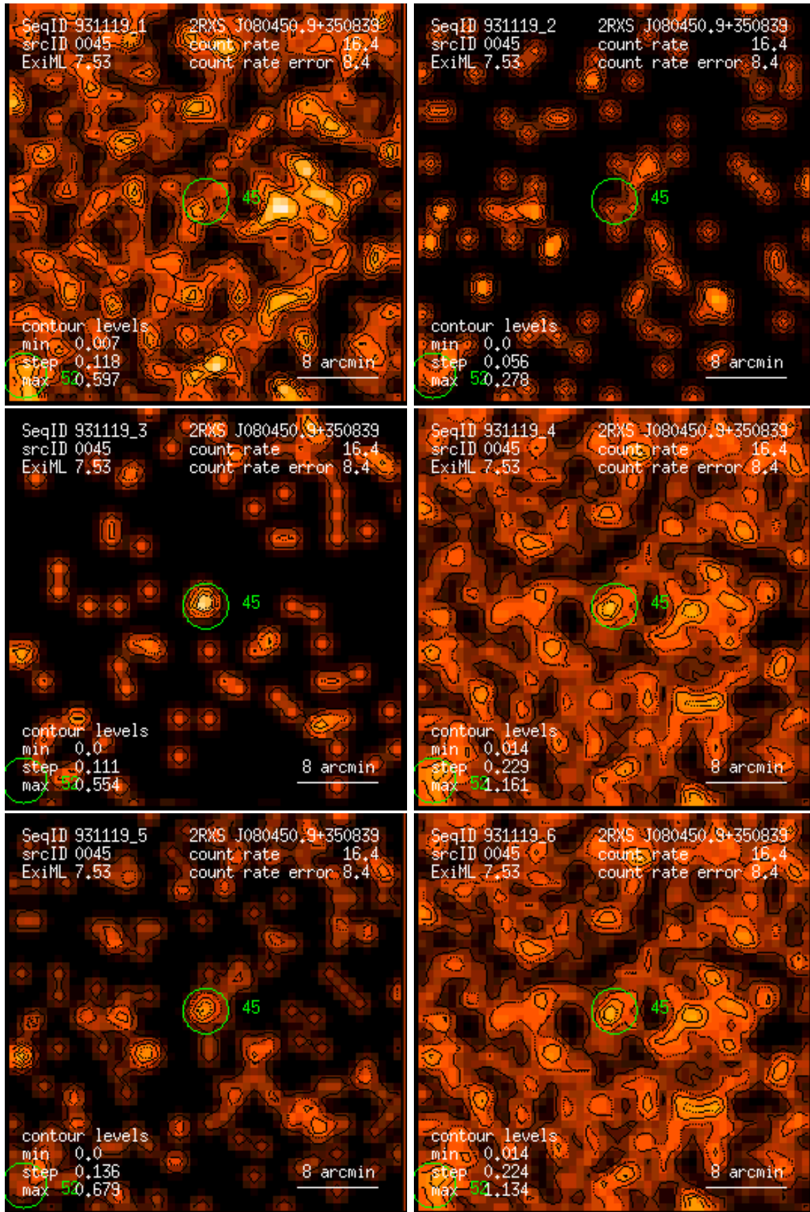
Figure 45: RASS 931119: detection 0045: band rate images, Gaussian filter: (1) PSPC channels 11 – 41, (2) 52 – 90, (3) 91 – 201, (4) 11 – 235, (5) 52 – 201, (6) 11 – 201. Broad band rates in counts/ks. Band rate contour levels in counts/ks/arcmin 2 .
