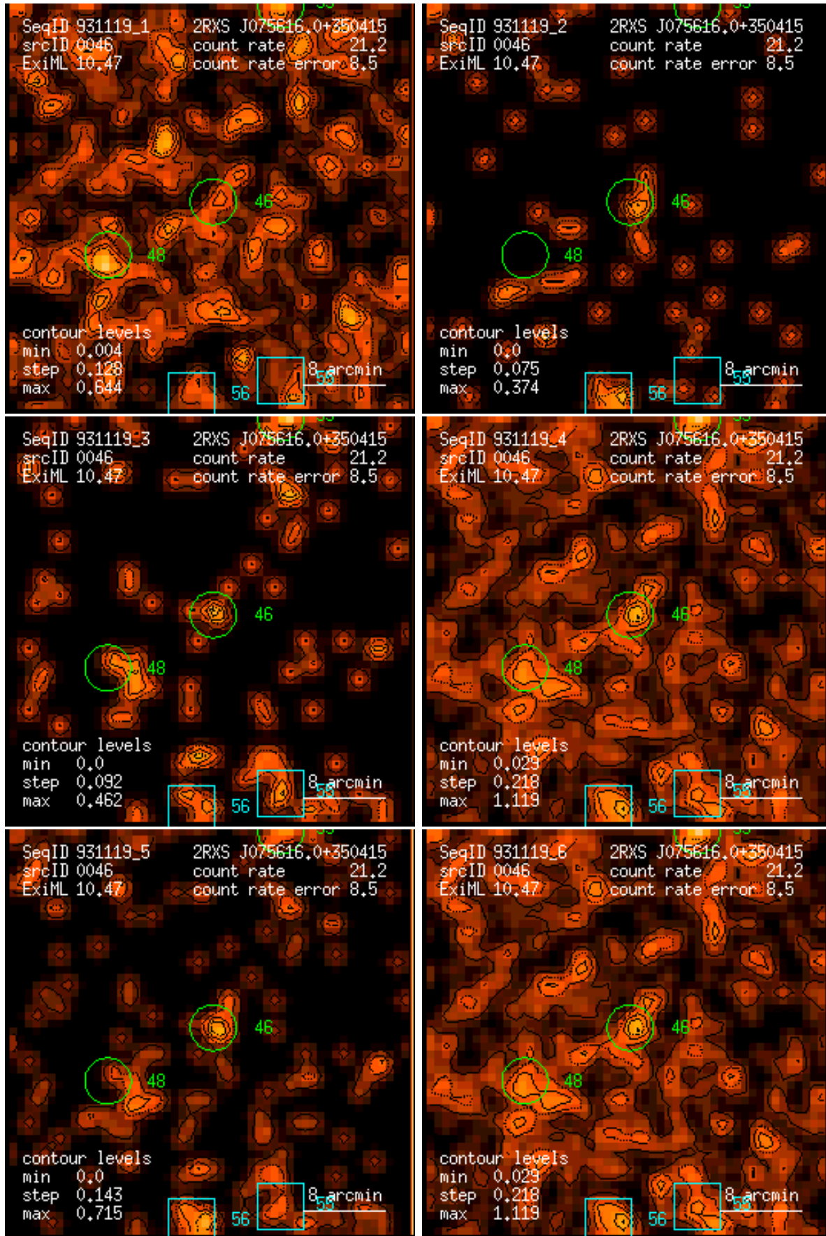
Figure 46: RASS 931119: detection 0046: band rate images, Gaussian filter: (1) PSPC channels 11 – 41, (2) 52 – 90, (3) 91 – 201, (4) 11 – 235, (5) 52 – 201, (6) 11 – 201. Broad band rates in counts/ks. Band rate contour levels in counts/ks/arcmin 2 .
