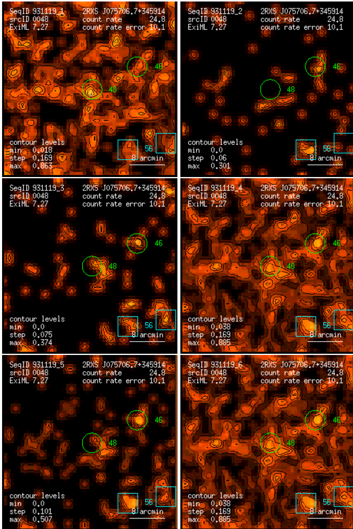
Figure 48: RASS 931119: detection 0048: band rate images, Gaussian filter: (1) PSPC channels 11 – 41, (2) 52 – 90, (3) 91 – 201, (4) 11 – 235, (5) 52 – 201, (6) 11 – 201. Broad band rates in counts/ks. Band rate contour levels in counts/ks/arcmin 2 .
