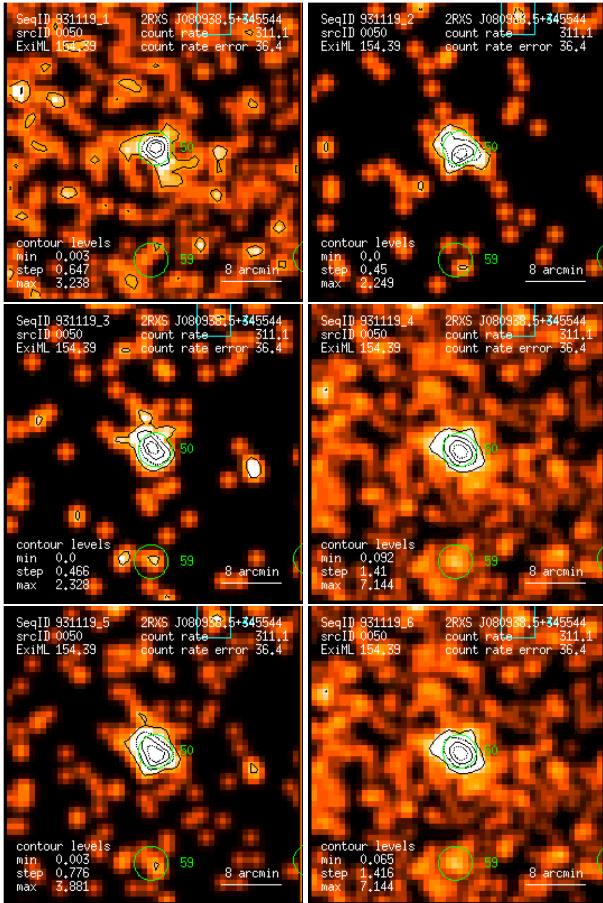
Figure 50: RASS 931119: detection 0050: band rate images, Gaussian filter: (1) PSPC channels 11 – 41, (2) 52 – 90, (3) 91 – 201, (4) 11 – 235, (5) 52 – 201, (6) 11 – 201. Broad band rates in counts/ks. Band rate contour levels in counts/ks/arcmin 2 .
