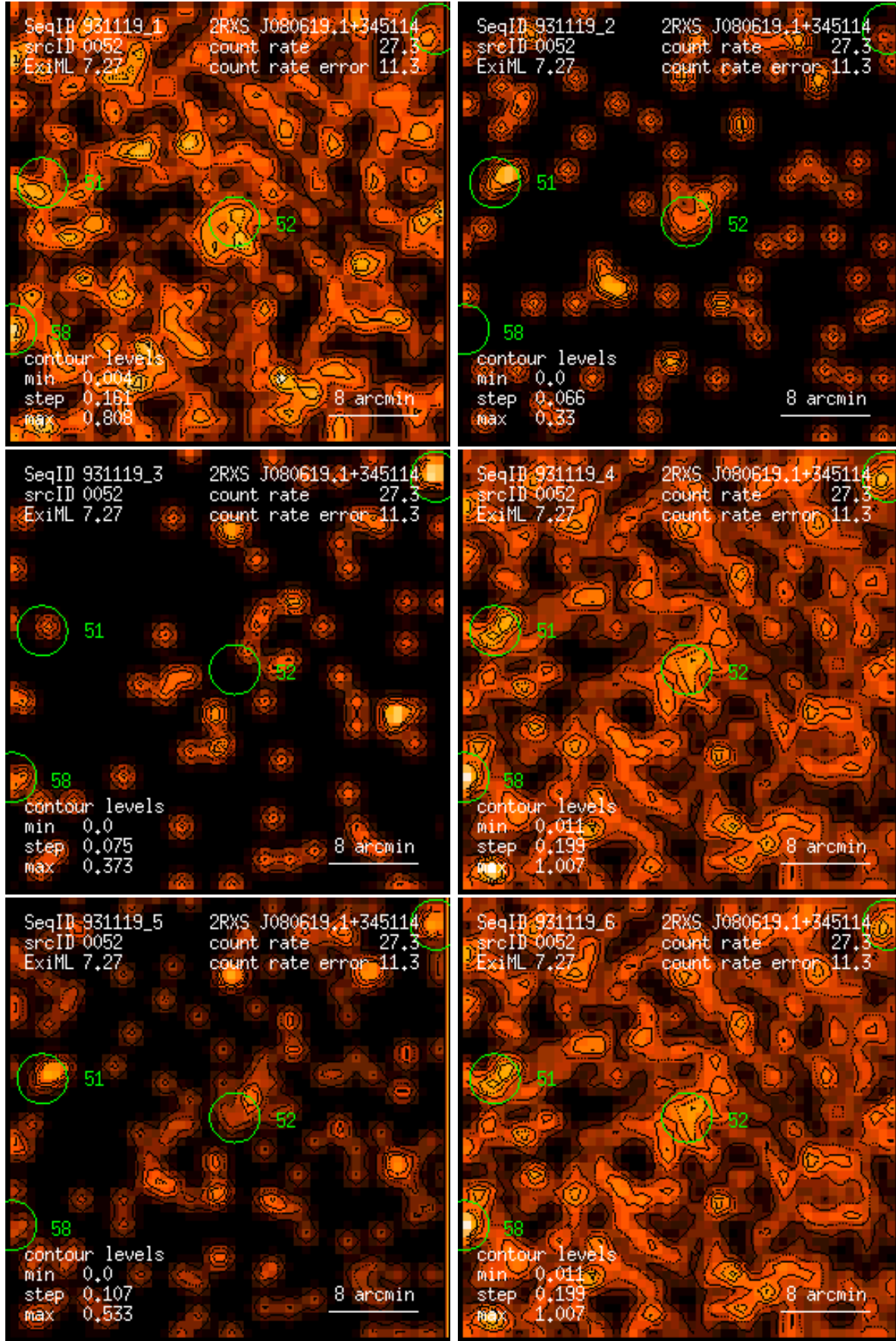
Figure 52: RASS 931119: detection 0052: band rate images, Gaussian filter: (1) PSPC channels 11 – 41, (2) 52 – 90, (3) 91 – 201, (4) 11 – 235, (5) 52 – 201, (6) 11 – 201. Broad band rates in counts/ks. Band rate contour levels in counts/ks/arcmin 2 .
