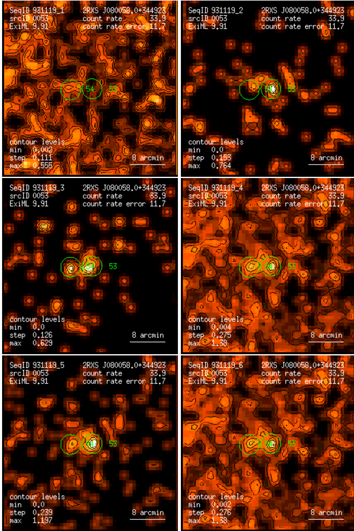
Figure 53: RASS 931119: detection 0053: band rate images, Gaussian filter: (1) PSPC channels 11 – 41, (2) 52 – 90, (3) 91 – 201, (4) 11 – 235, (5) 52 – 201, (6) 11 – 201. Broad band rates in counts/ks. Band rate contour levels in counts/ks/arcmin 2 .
