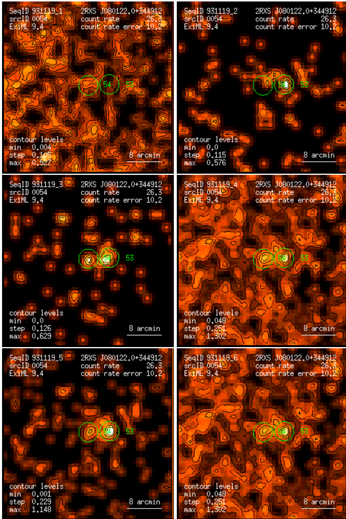
Figure 54: RASS 931119: detection 0054: band rate images, Gaussian filter: (1) PSPC channels 11 – 41, (2) 52 – 90, (3) 91 – 201, (4) 11 – 235, (5) 52 – 201, (6) 11 – 201. Broad band rates in counts/ks. Band rate contour levels in counts/ks/arcmin 2 .
