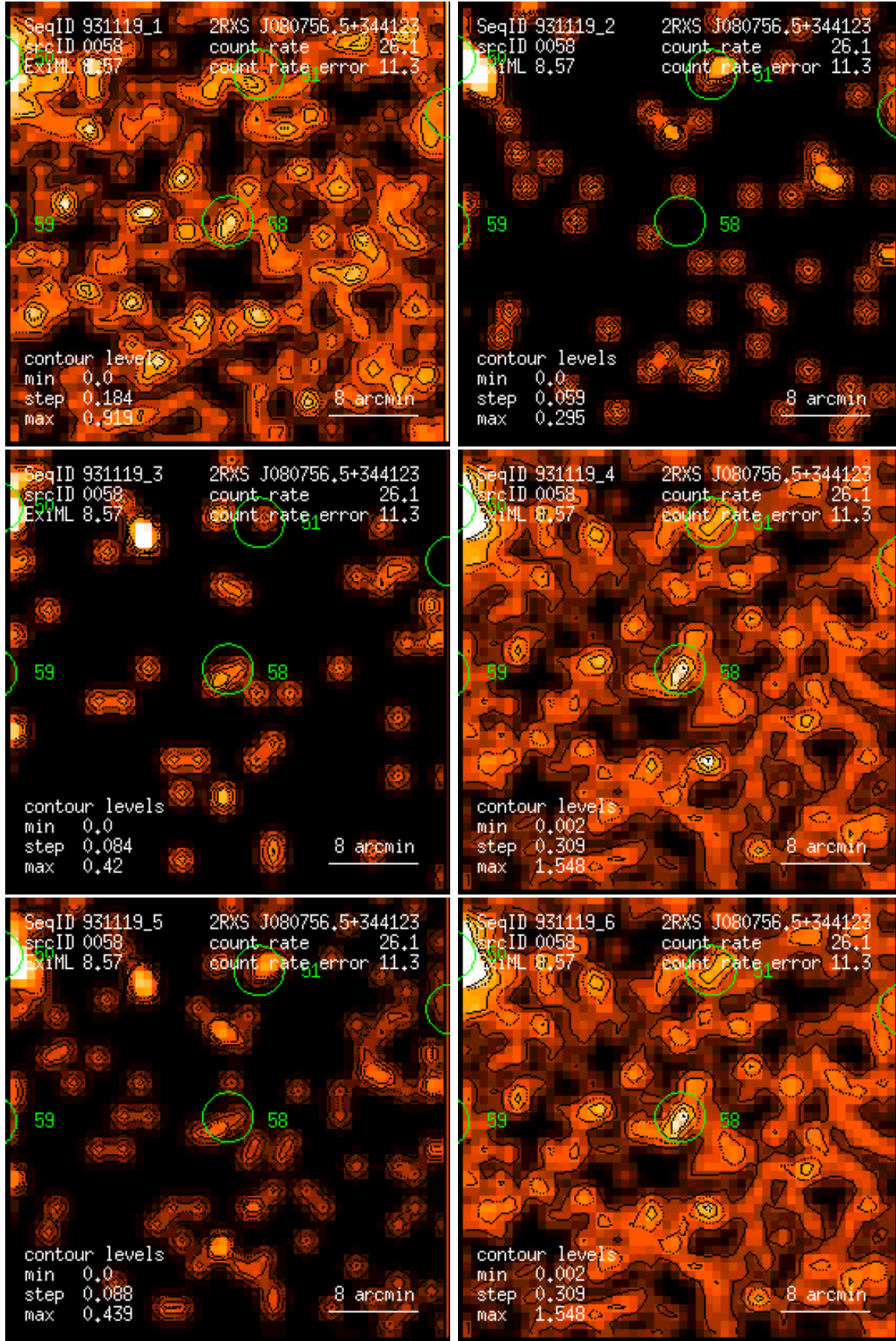
Figure 58: RASS 931119: detection 0058: band rate images, Gaussian filter: (1) PSPC channels 11 – 41, (2) 52 – 90, (3) 91 – 201, (4) 11 – 235, (5) 52 – 201, (6) 11 – 201. Broad band rates in counts/ks. Band rate contour levels in counts/ks/arcmin 2 .
