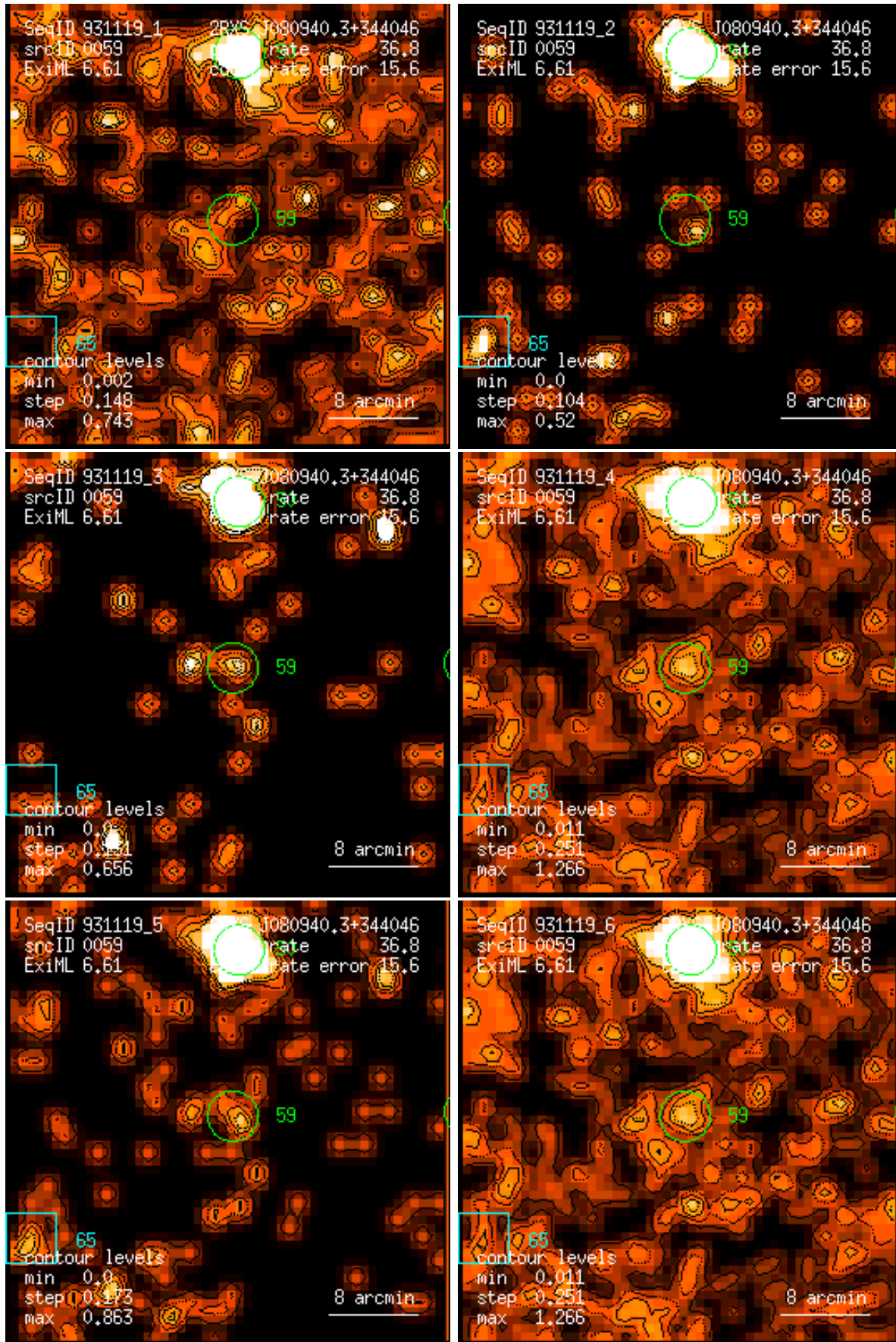
Figure 59: RASS 931119: detection 0059: band rate images, Gaussian filter: (1) PSPC channels 11 – 41, (2) 52 – 90, (3) 91 – 201, (4) 11 – 235, (5) 52 – 201, (6) 11 – 201. Broad band rates in counts/ks. Band rate contour levels in counts/ks/arcmin 2 .
