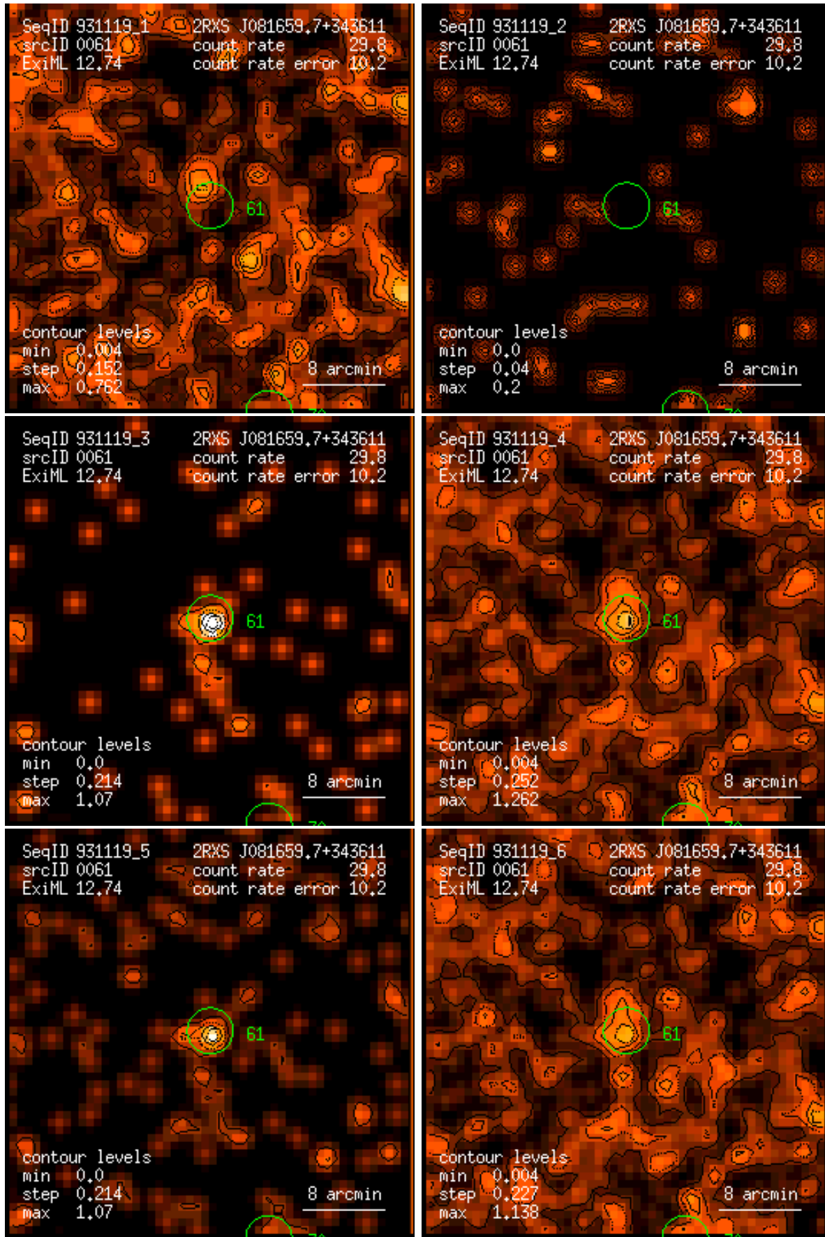
Figure 61: RASS 931119: detection 0061: band rate images, Gaussian filter: (1) PSPC channels 11 – 41, (2) 52 – 90, (3) 91 – 201, (4) 11 – 235, (5) 52 – 201, (6) 11 – 201. Broad band rates in counts/ks. Band rate contour levels in counts/ks/arcmin 2 .
