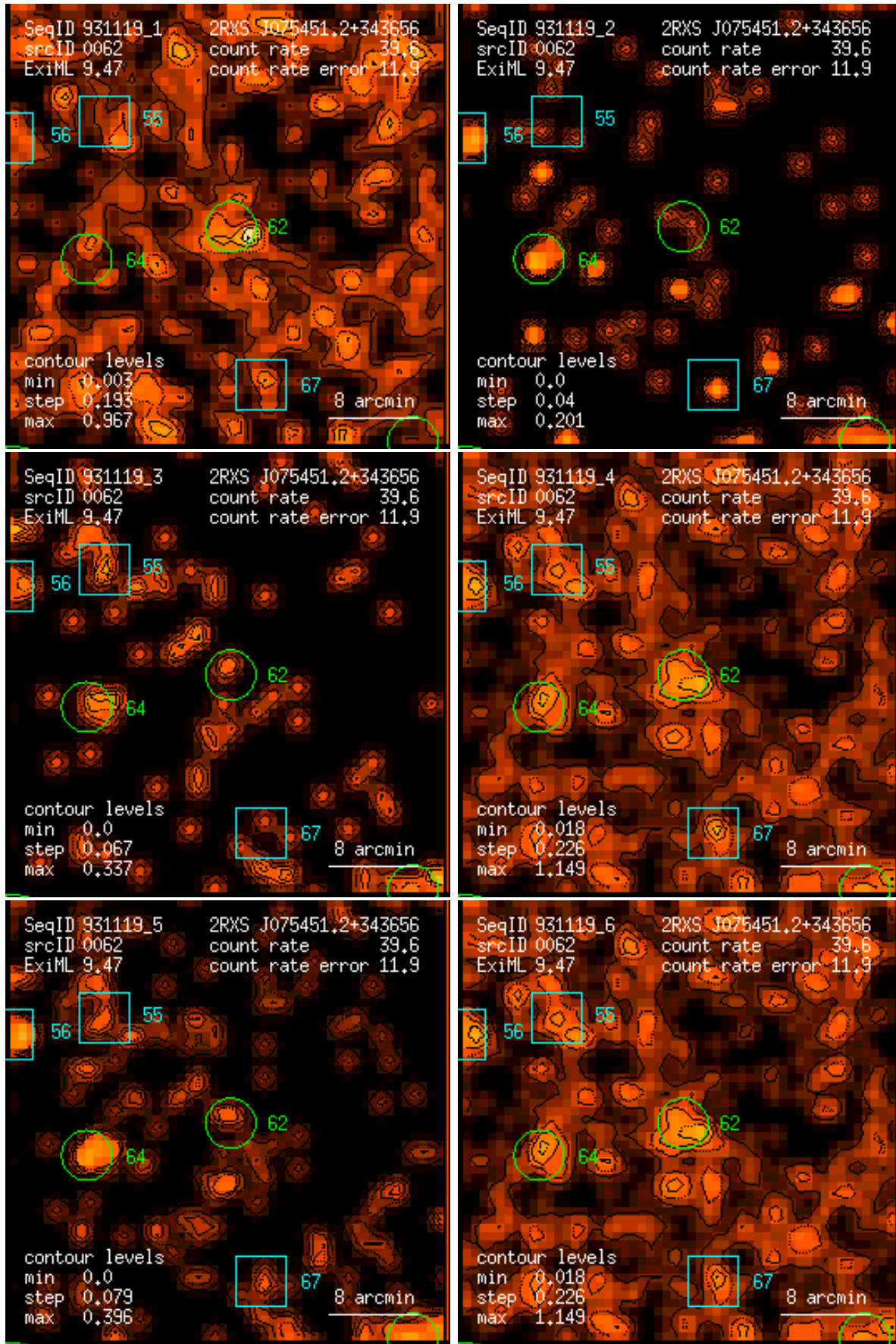
Figure 62: RASS 931119: detection 0062: band rate images, Gaussian filter: (1) PSPC channels 11 – 41, (2) 52 – 90, (3) 91 – 201, (4) 11 – 235, (5) 52 – 201, (6) 11 – 201. Broad band rates in counts/ks. Band rate contour levels in counts/ks/arcmin 2 .
