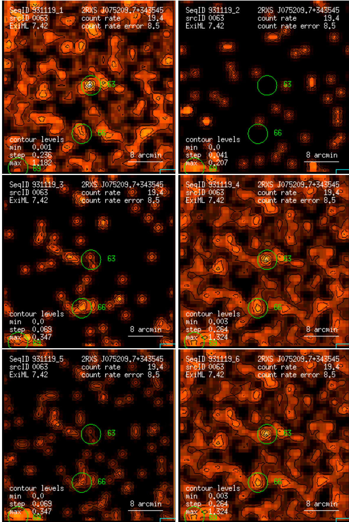
Figure 63: RASS 931119: detection 0063: band rate images, Gaussian filter: (1) PSPC channels 11 – 41, (2) 52 – 90, (3) 91 – 201, (4) 11 – 235, (5) 52 – 201, (6) 11 – 201. Broad band rates in counts/ks. Band rate contour levels in counts/ks/arcmin 2 .
