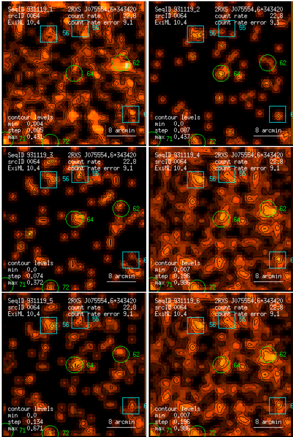
Figure 64: RASS 931119: detection 0064: band rate images, Gaussian filter: (1) PSPC channels 11 – 41, (2) 52 – 90, (3) 91 – 201, (4) 11 – 235, (5) 52 – 201, (6) 11 – 201. Broad band rates in counts/ks. Band rate contour levels in counts/ks/arcmin 2 .
