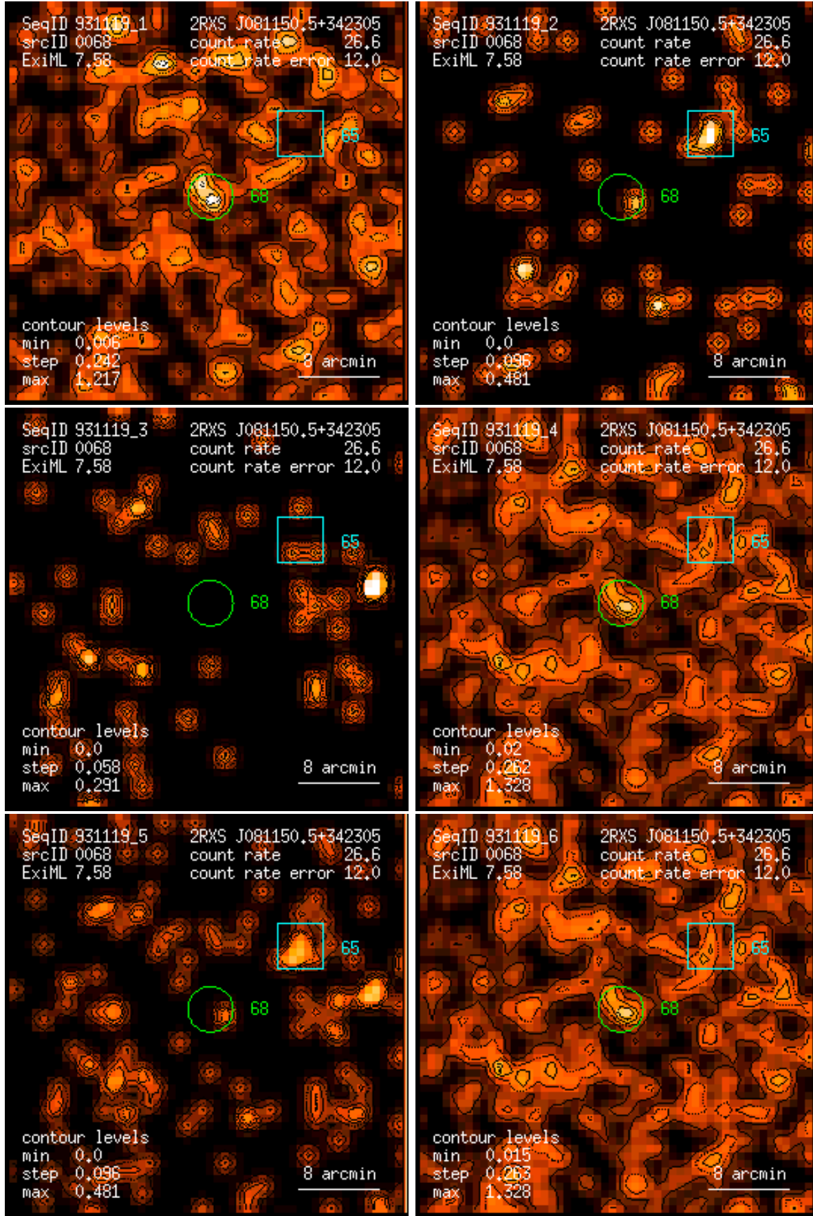
Figure 68: RASS 931119: detection 0068: band rate images, Gaussian filter: (1) PSPC channels 11 – 41, (2) 52 – 90, (3) 91 – 201, (4) 11 – 235, (5) 52 – 201, (6) 11 – 201. Broad band rates in counts/ks. Band rate contour levels in counts/ks/arcmin 2 .
