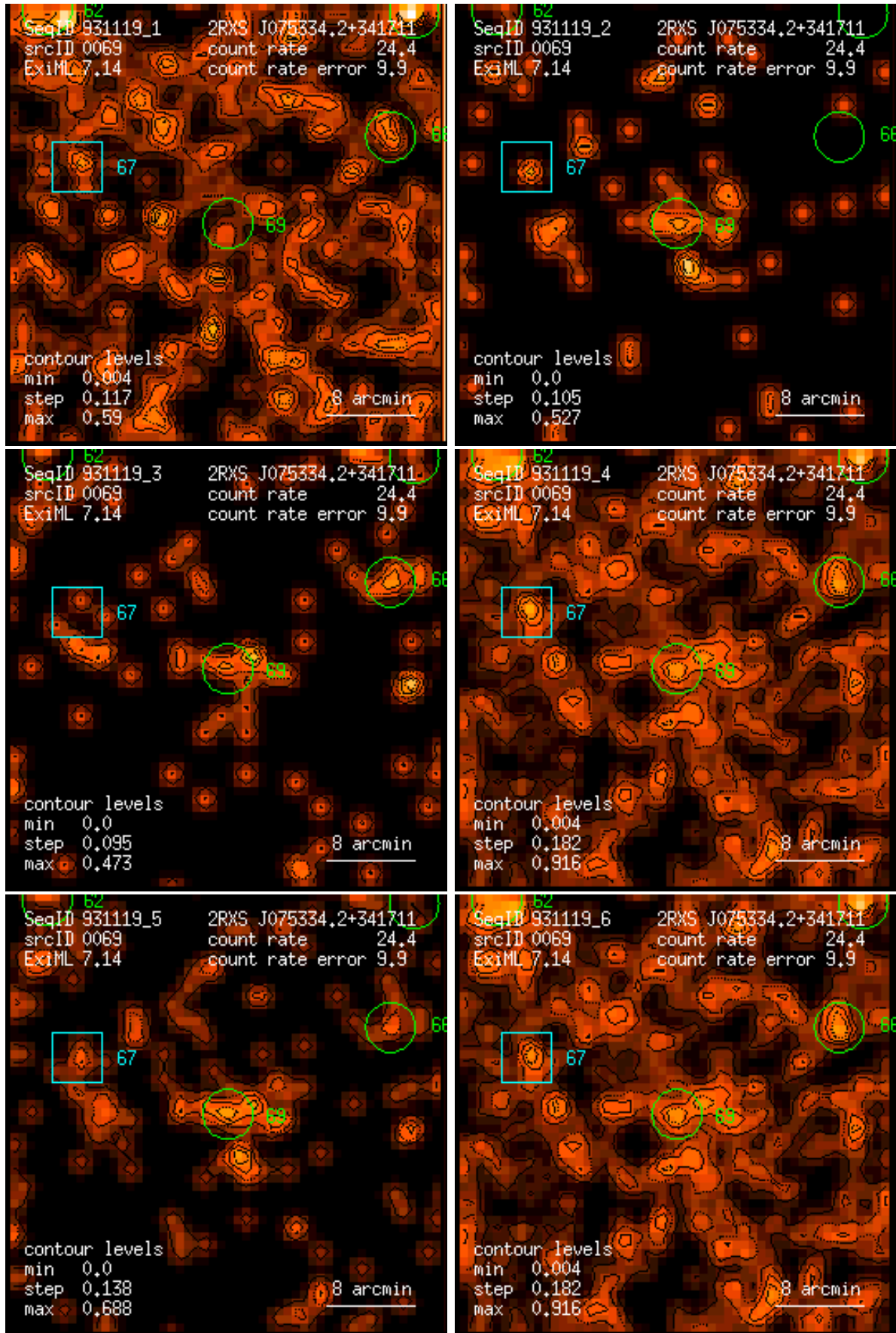
Figure 69: RASS 931119: detection 0069: band rate images, Gaussian filter: (1) PSPC channels 11 – 41, (2) 52 – 90, (3) 91 – 201, (4) 11 – 235, (5) 52 – 201, (6) 11 – 201. Broad band rates in counts/ks. Band rate contour levels in counts/ks/arcmin 2 .
