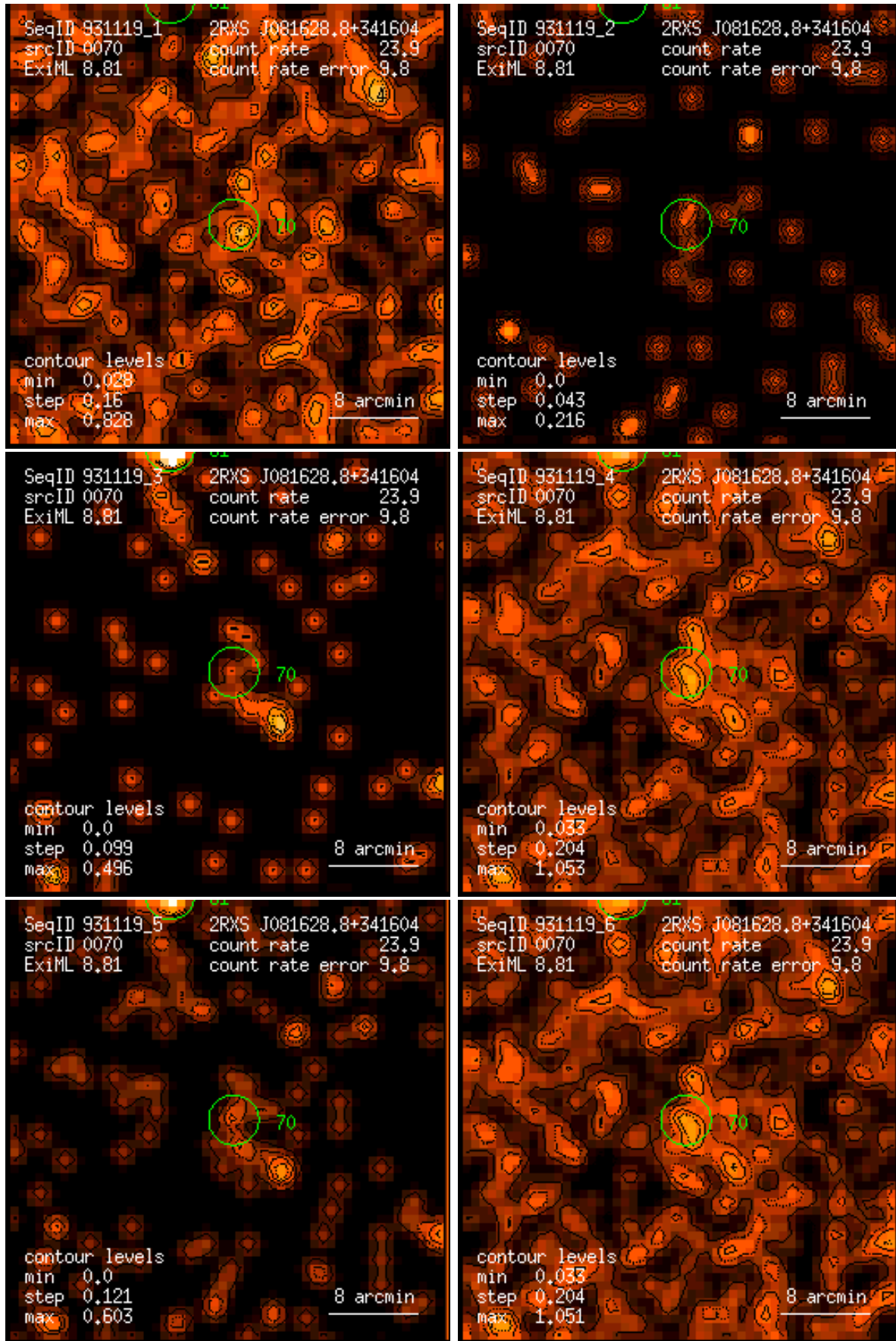
Figure 70: RASS 931119: detection 0070: band rate images, Gaussian filter: (1) PSPC channels 11 – 41, (2) 52 – 90, (3) 91 – 201, (4) 11 – 235, (5) 52 – 201, (6) 11 – 201. Broad band rates in counts/ks. Band rate contour levels in counts/ks/arcmin 2 .
