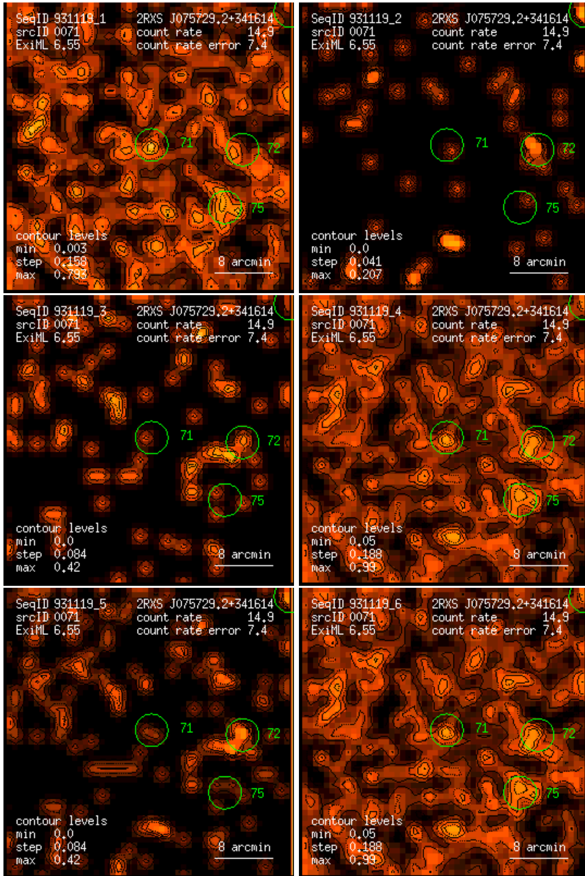
Figure 71: RASS 931119: detection 0071: band rate images, Gaussian filter: (1) PSPC channels 11 – 41, (2) 52 – 90, (3) 91 – 201, (4) 11 – 235, (5) 52 – 201, (6) 11 – 201. Broad band rates in counts/ks. Band rate contour levels in counts/ks/arcmin 2 .
