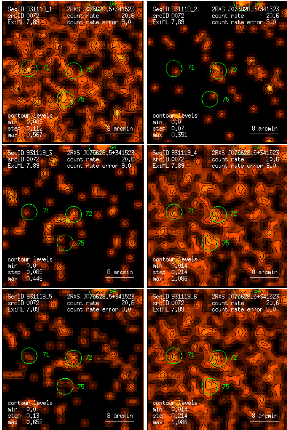
Figure 72: RASS 931119: detection 0072: band rate images, Gaussian filter: (1) PSPC channels 11 – 41, (2) 52 – 90, (3) 91 – 201, (4) 11 – 235, (5) 52 – 201, (6) 11 – 201. Broad band rates in counts/ks. Band rate contour levels in counts/ks/arcmin 2 .
