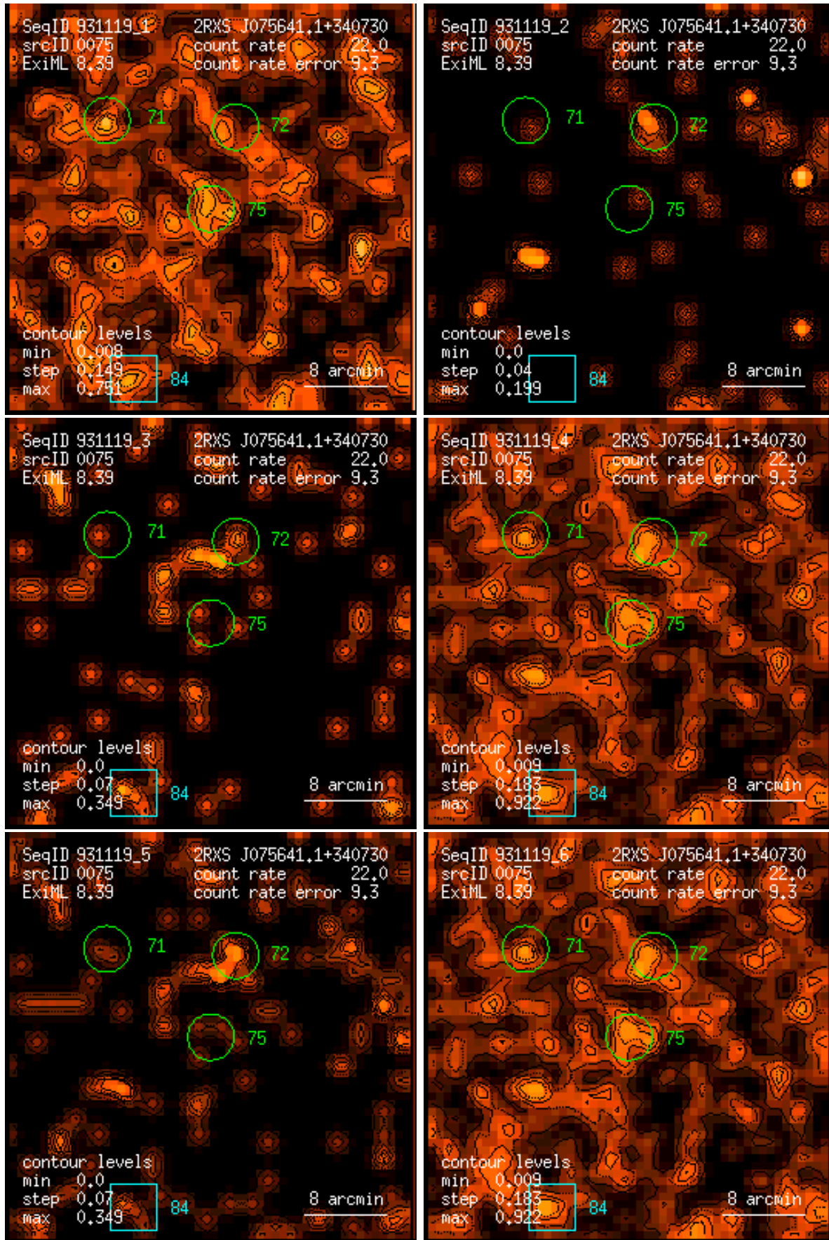
Figure 75: RASS 931119: detection 0075: band rate images, Gaussian filter: (1) PSPC channels 11 – 41, (2) 52 – 90, (3) 91 – 201, (4) 11 – 235, (5) 52 – 201, (6) 11 – 201. Broad band rates in counts/ks. Band rate contour levels in counts/ks/arcmin 2 .
