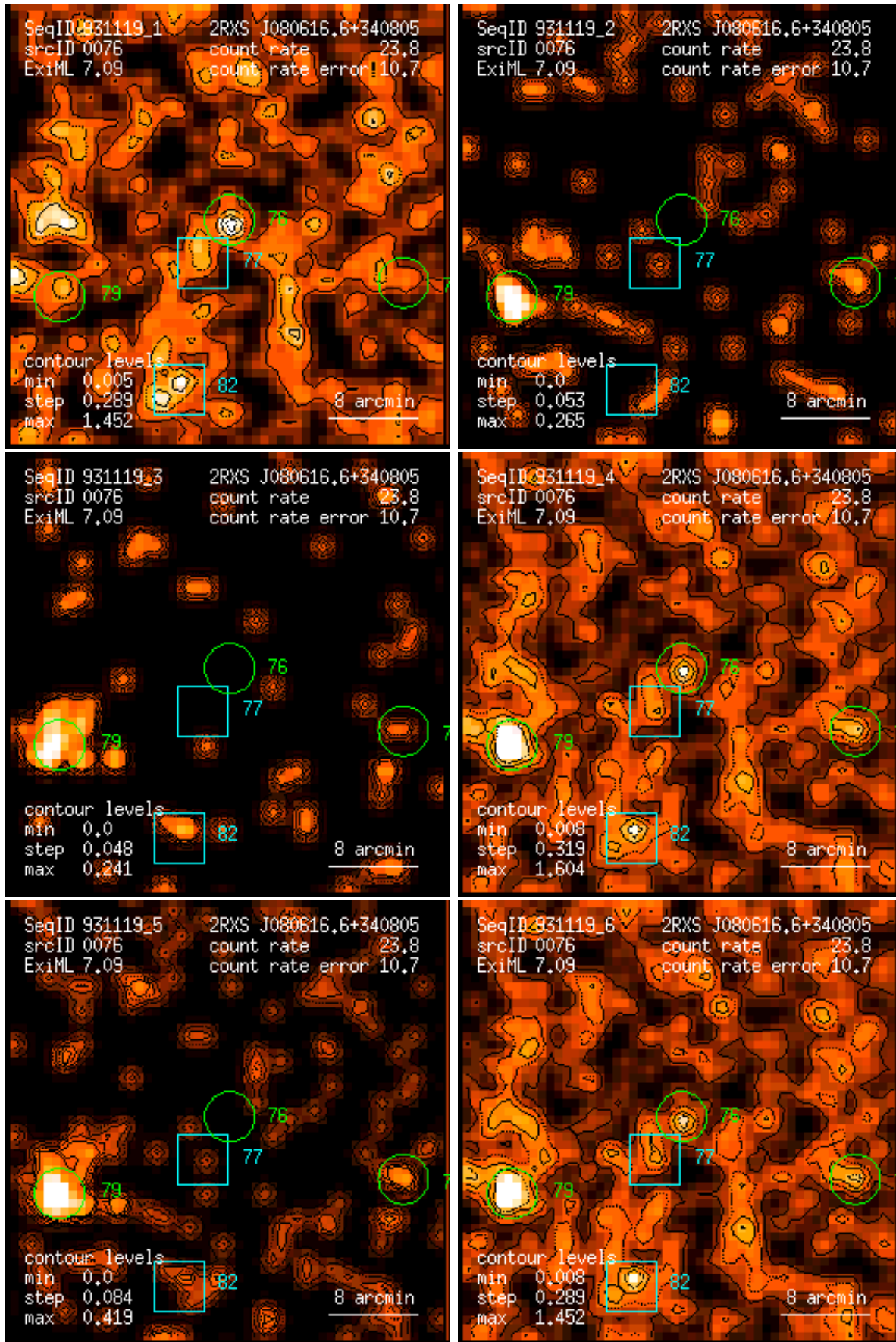
Figure 76: RASS 931119: detection 0076: band rate images, Gaussian filter: (1) PSPC channels 11 – 41, (2) 52 – 90, (3) 91 – 201, (4) 11 – 235, (5) 52 – 201, (6) 11 – 201. Broad band rates in counts/ks. Band rate contour levels in counts/ks/arcmin 2 .
