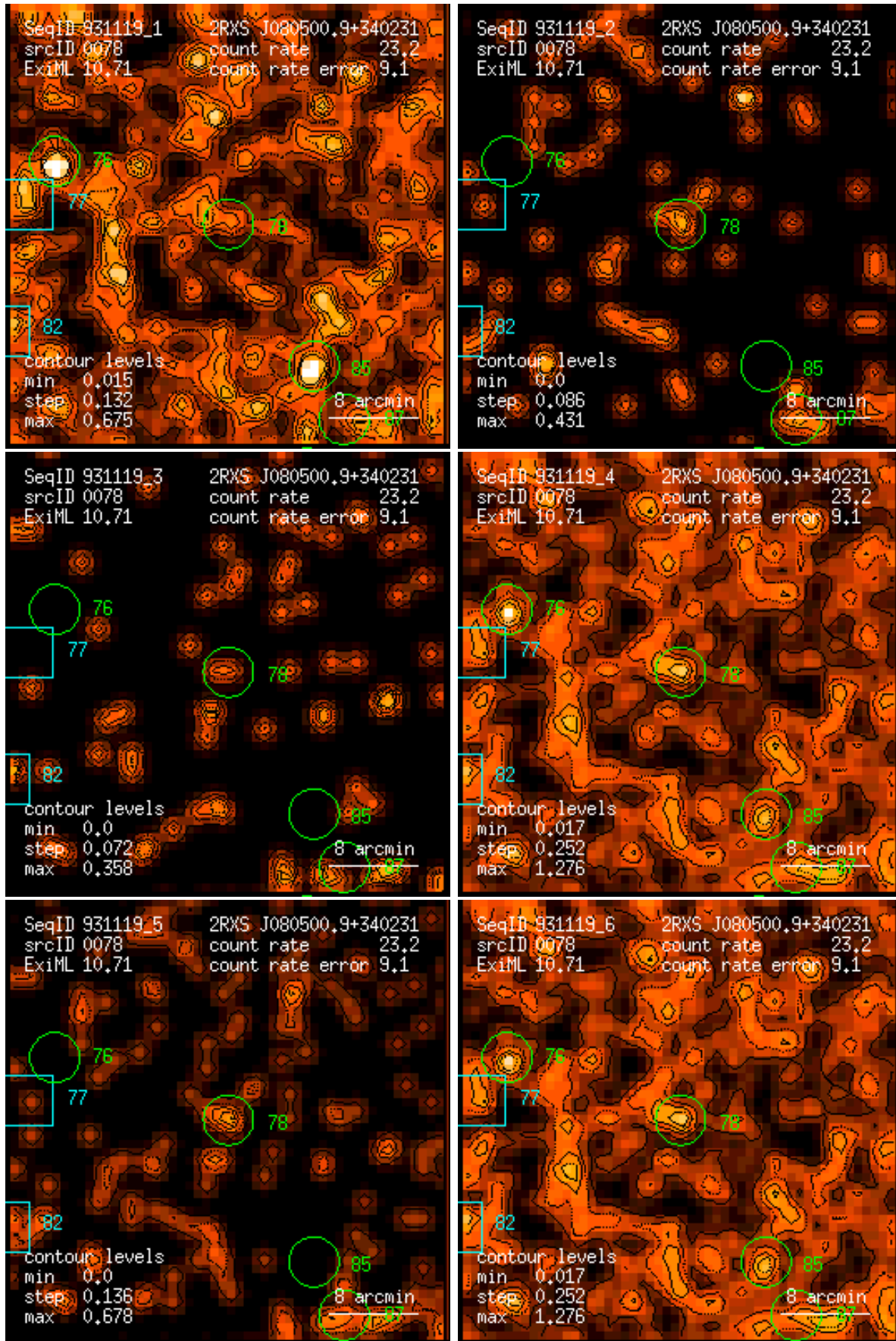
Figure 78: RASS 931119: detection 0078: band rate images, Gaussian filter: (1) PSPC channels 11 – 41, (2) 52 – 90, (3) 91 – 201, (4) 11 – 235, (5) 52 – 201, (6) 11 – 201. Broad band rates in counts/ks. Band rate contour levels in counts/ks/arcmin 2 .
