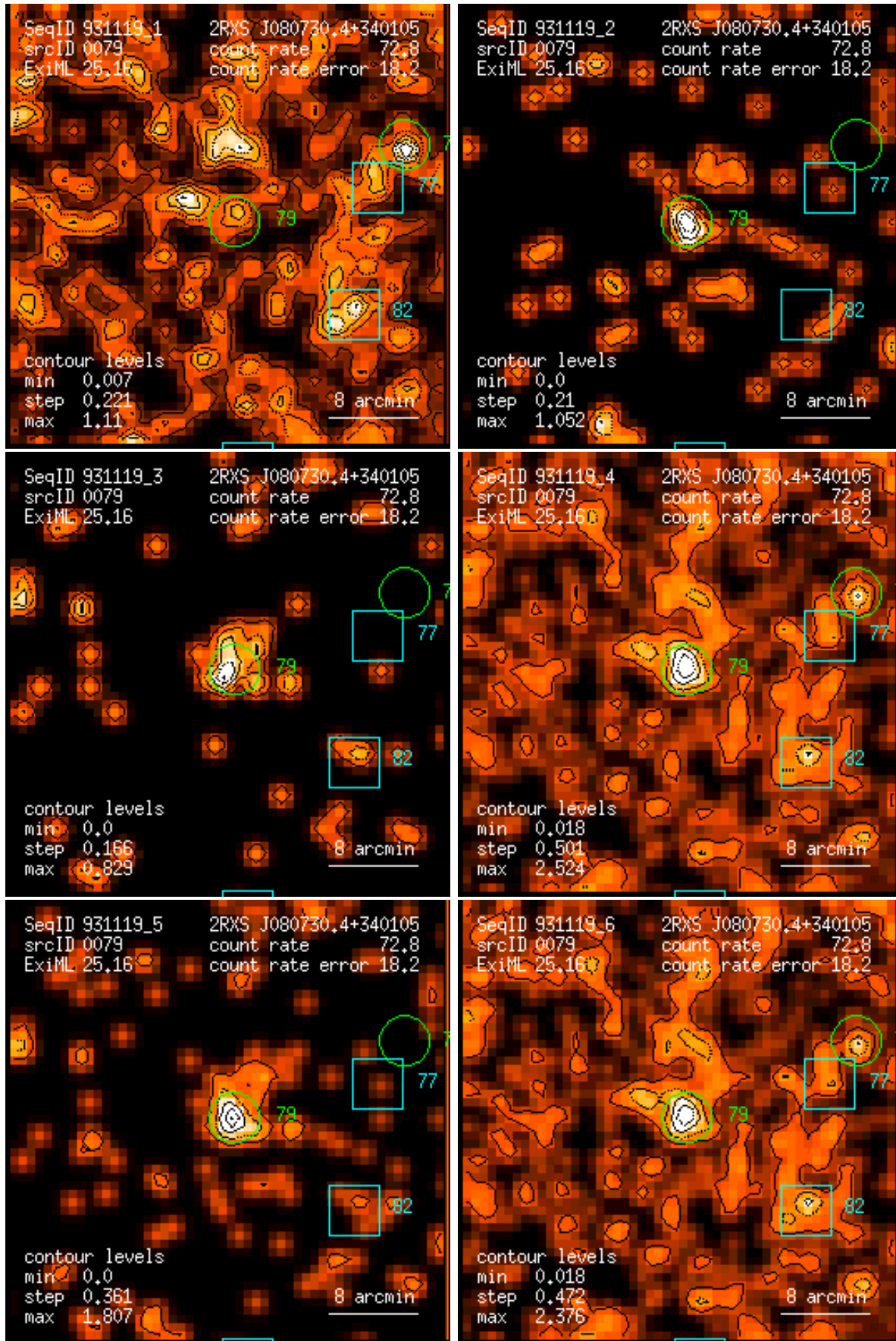
Figure 79: RASS 931119: detection 0079: band rate images, Gaussian filter: (1) PSPC channels 11 – 41, (2) 52 – 90, (3) 91 – 201, (4) 11 – 235, (5) 52 – 201, (6) 11 – 201. Broad band rates in counts/ks. Band rate contour levels in counts/ks/arcmin 2 .
