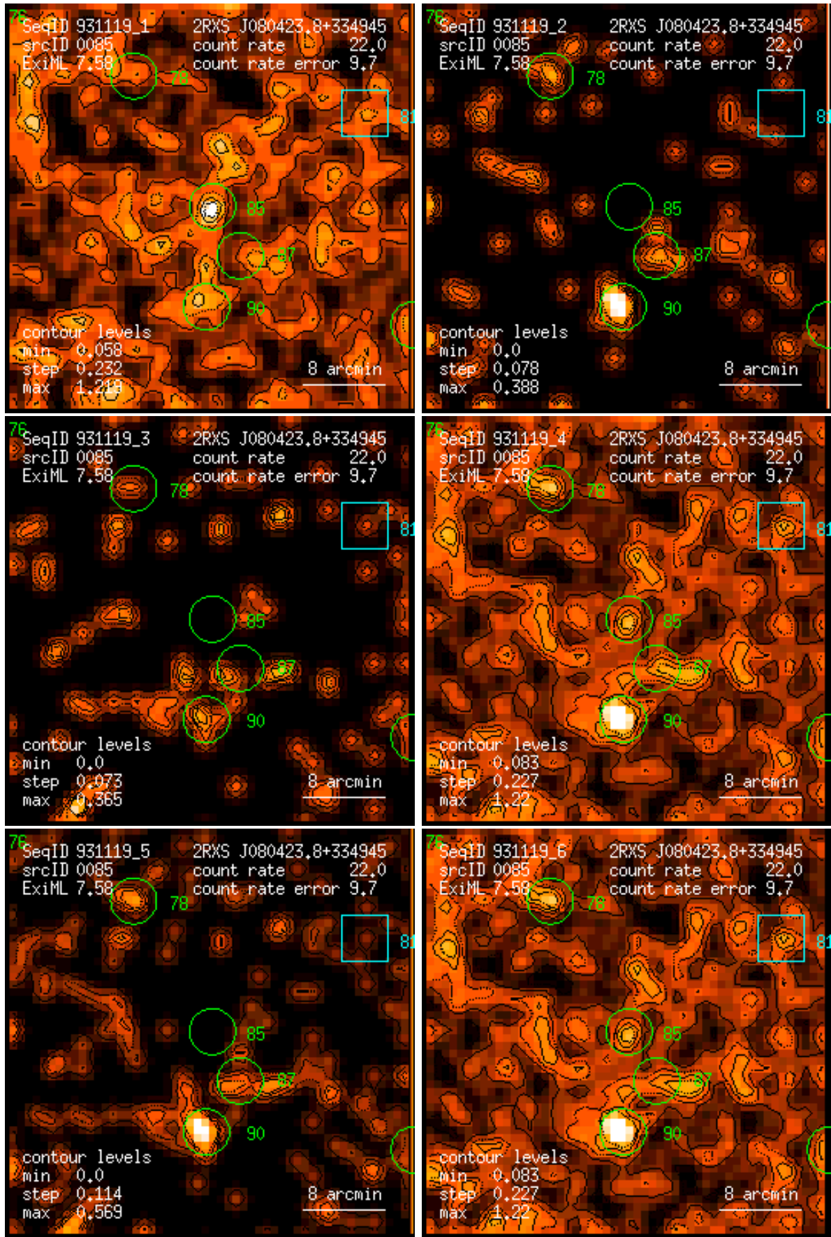
Figure 85: RASS 931119: detection 0085: band rate images, Gaussian filter: (1) PSPC channels 11 – 41, (2) 52 – 90, (3) 91 – 201, (4) 11 – 235, (5) 52 – 201, (6) 11 – 201. Broad band rates in counts/ks. Band rate contour levels in counts/ks/arcmin 2 .
