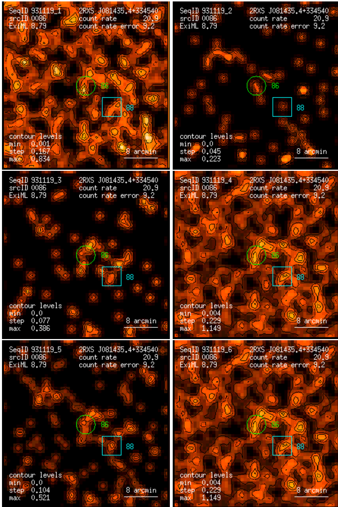
Figure 86: RASS 931119: detection 0086: band rate images, Gaussian filter: (1) PSPC channels 11 – 41, (2) 52 – 90, (3) 91 – 201, (4) 11 – 235, (5) 52 – 201, (6) 11 – 201. Broad band rates in counts/ks. Band rate contour levels in counts/ks/arcmin 2 .
