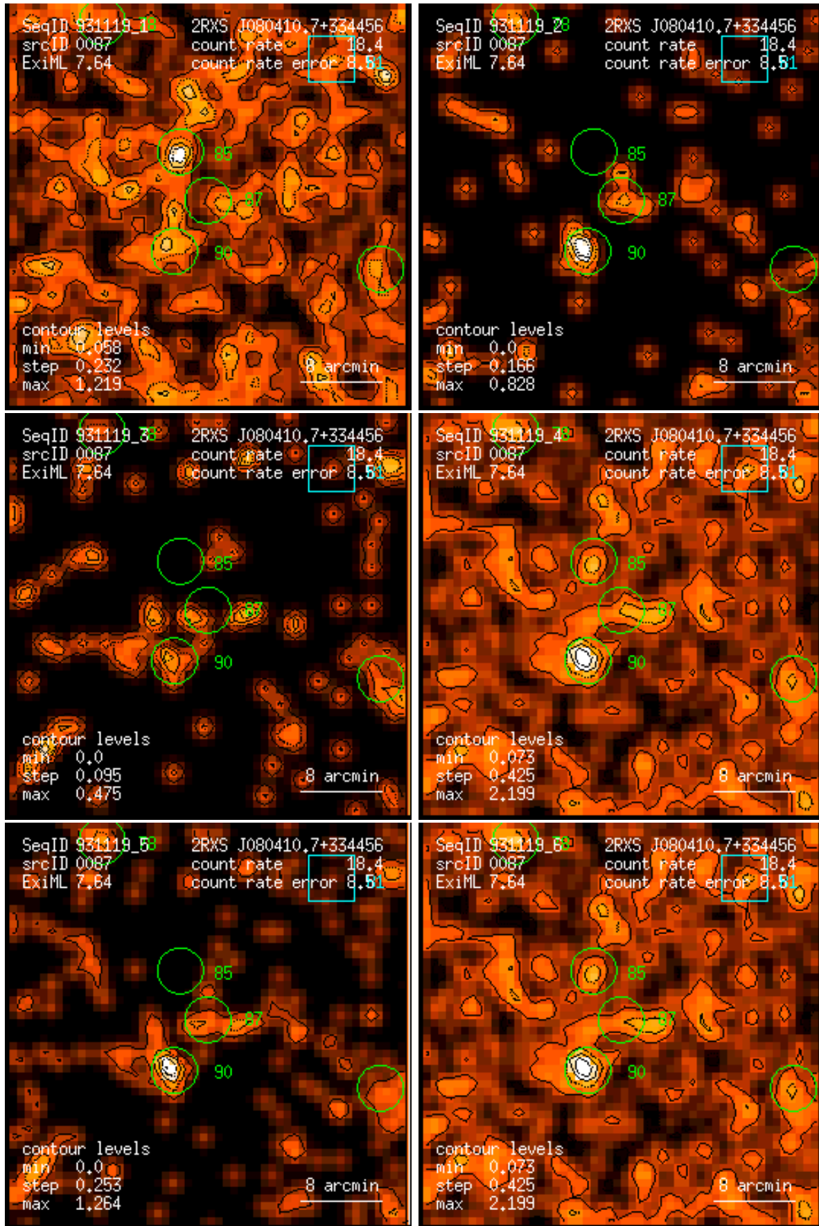
Figure 87: RASS 931119: detection 0087: band rate images, Gaussian filter: (1) PSPC channels 11 – 41, (2) 52 – 90, (3) 91 – 201, (4) 11 – 235, (5) 52 – 201, (6) 11 – 201. Broad band rates in counts/ks. Band rate contour levels in counts/ks/arcmin 2 .
