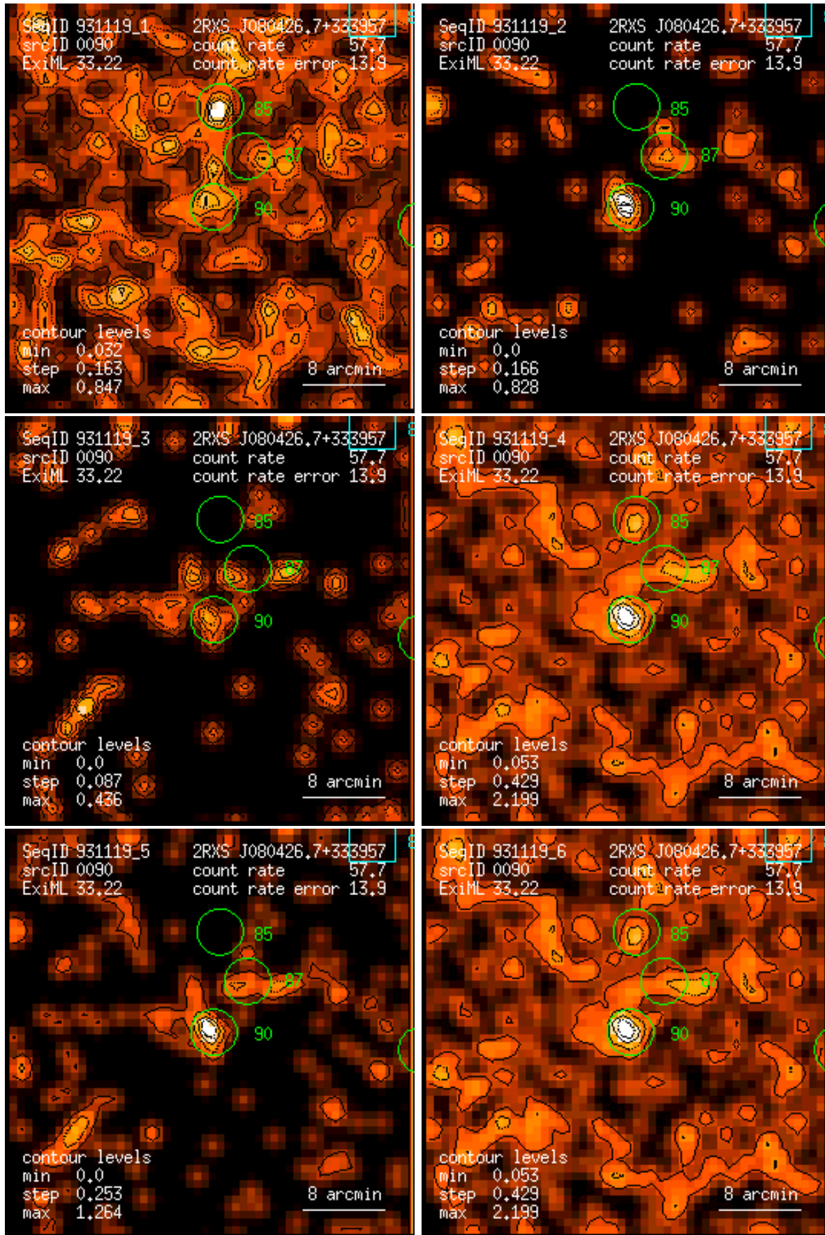
Figure 90: RASS 931119: detection 0090: band rate images, Gaussian filter: (1) PSPC channels 11 – 41, (2) 52 – 90, (3) 91 – 201, (4) 11 – 235, (5) 52 – 201, (6) 11 – 201. Broad band rates in counts/ks. Band rate contour levels in counts/ks/arcmin 2 .
