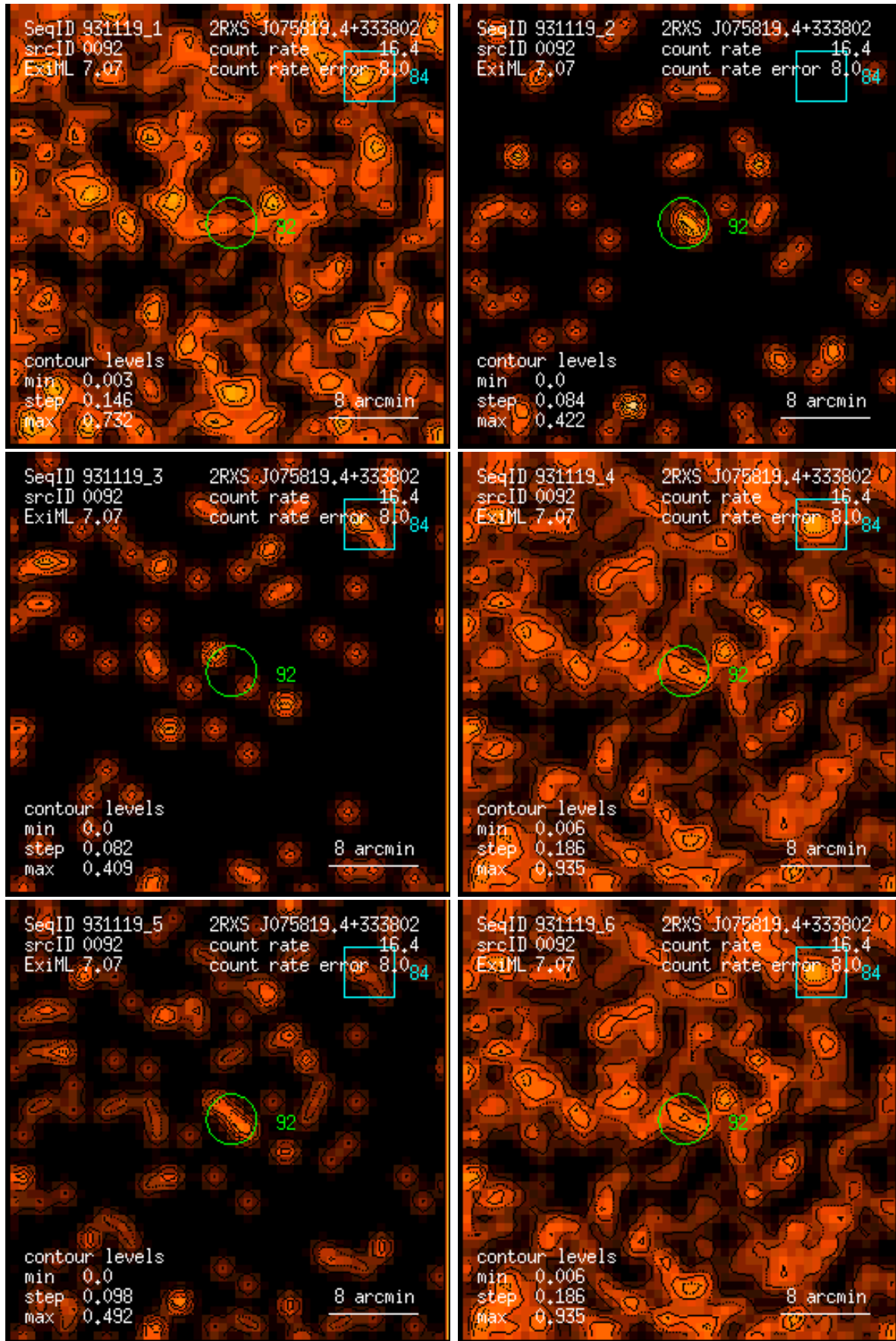
Figure 92: RASS 931119: detection 0092: band rate images, Gaussian filter: (1) PSPC channels 11 – 41, (2) 52 – 90, (3) 91 – 201, (4) 11 – 235, (5) 52 – 201, (6) 11 – 201. Broad band rates in counts/ks. Band rate contour levels in counts/ks/arcmin 2 .
