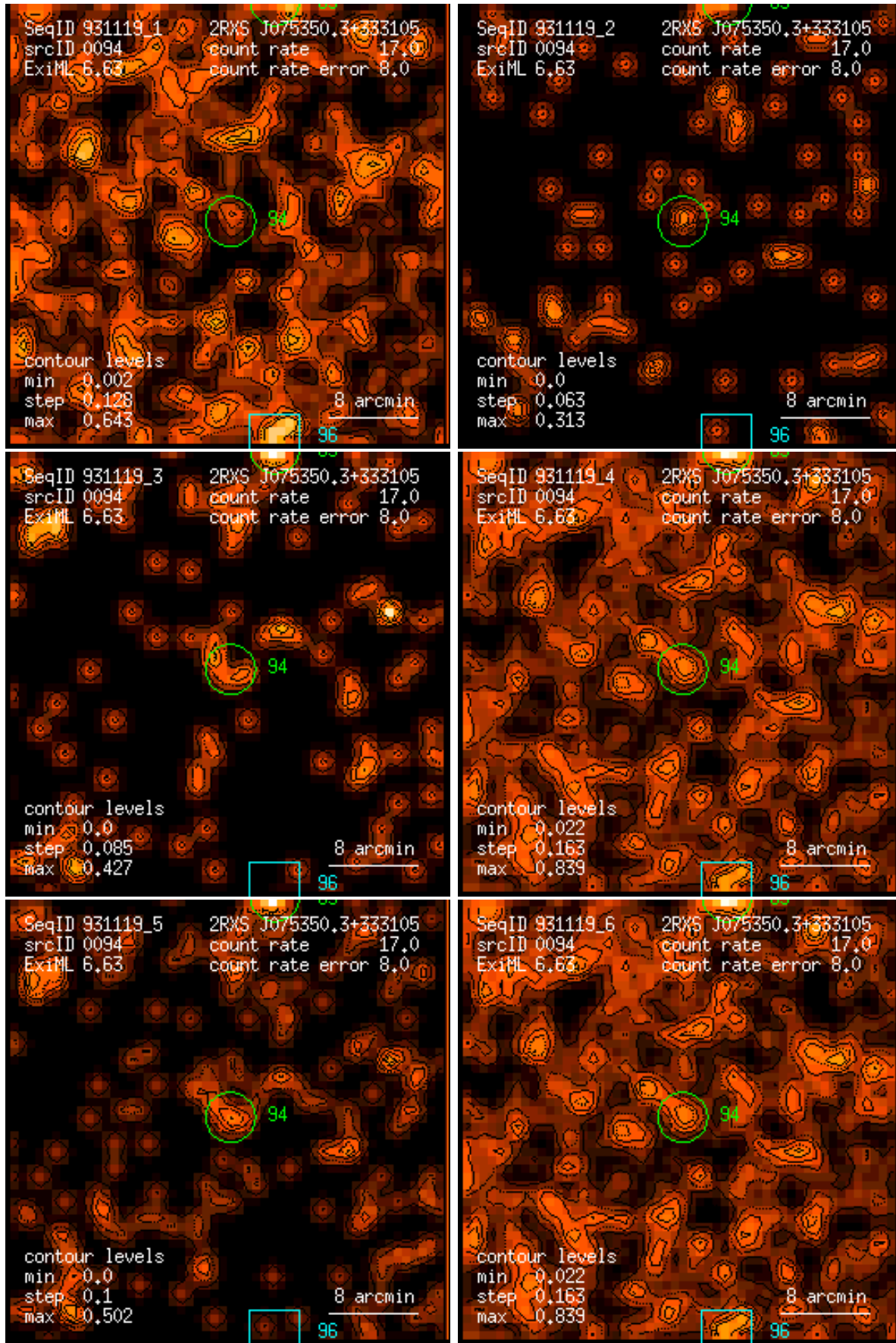
Figure 94: RASS 931119: detection 0094: band rate images, Gaussian filter: (1) PSPC channels 11 – 41, (2) 52 – 90, (3) 91 – 201, (4) 11 – 235, (5) 52 – 201, (6) 11 – 201. Broad band rates in counts/ks. Band rate contour levels in counts/ks/arcmin 2 .
