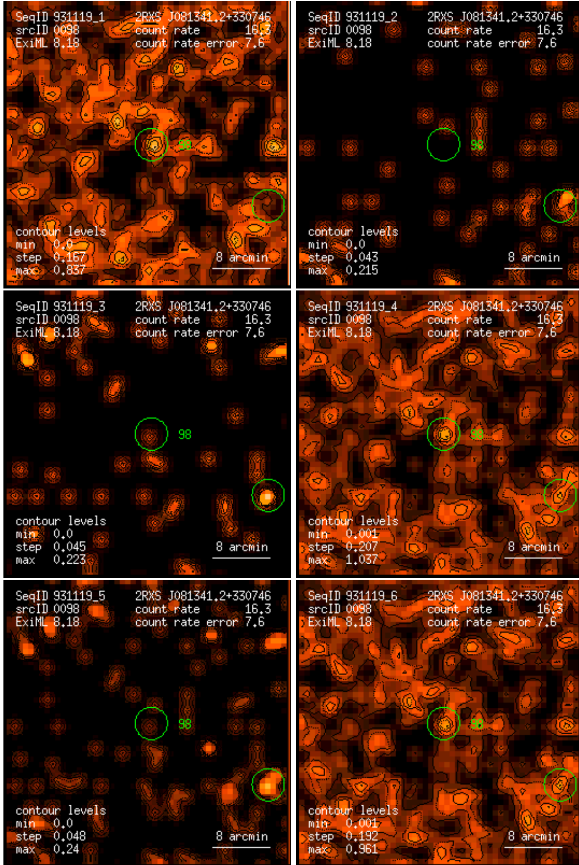
Figure 98: RASS 931119: detection 0098: band rate images, Gaussian filter: (1) PSPC channels 11 – 41, (2) 52 – 90, (3) 91 – 201, (4) 11 – 235, (5) 52 – 201, (6) 11 – 201. Broad band rates in counts/ks. Band rate contour levels in counts/ks/arcmin 2 .
