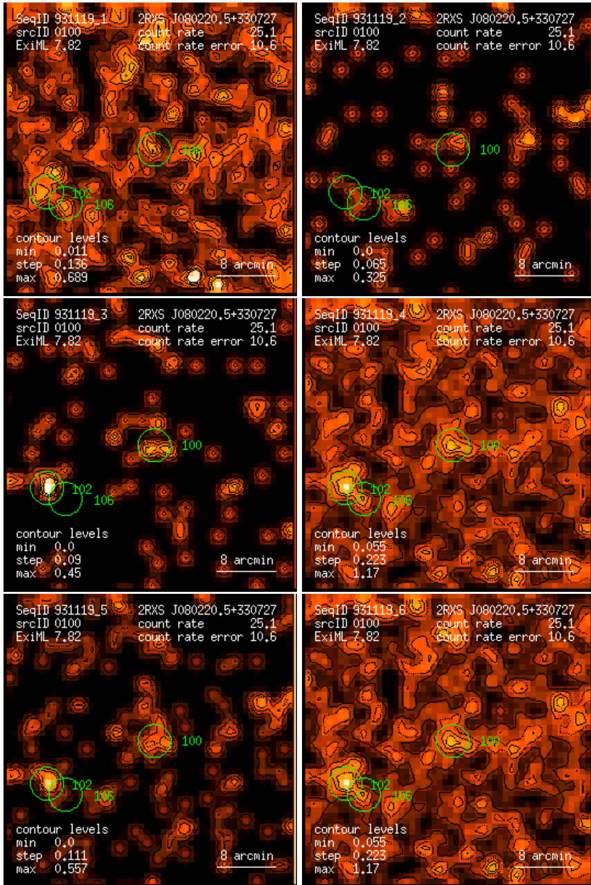
Figure 100: RASS 931119: detection 0100: band rate images, Gaussian filter: (1) PSPC channels 11 – 41, (2) 52 – 90, (3) 91 – 201, (4) 11 – 235, (5) 52 – 201, (6) 11 – 201. Broad band rates in counts/ks. Band rate contour levels in counts/ks/arcmin 2 .
