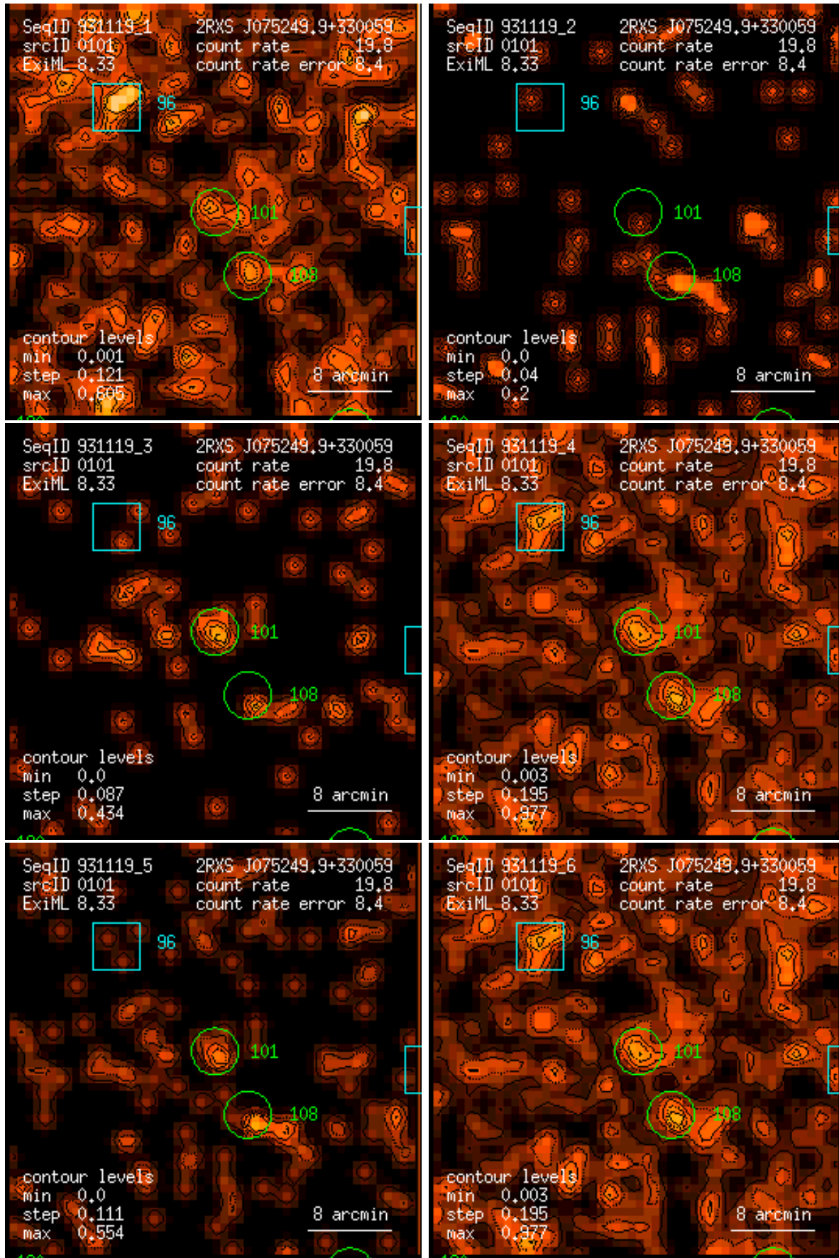
Figure 101: RASS 931119: detection 0101: band rate images, Gaussian filter: (1) PSPC channels 11 – 41, (2) 52 – 90, (3) 91 – 201, (4) 11 – 235, (5) 52 – 201, (6) 11 – 201. Broad band rates in counts/ks. Band rate contour levels in counts/ks/arcmin 2 .
