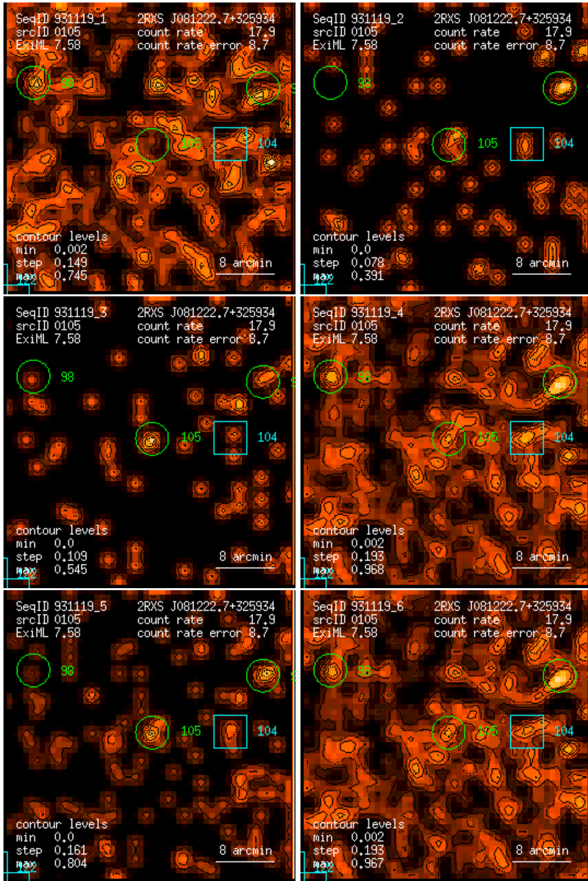
Figure 105: RASS 931119: detection 0105: band rate images, Gaussian filter: (1) PSPC channels 11 – 41, (2) 52 – 90, (3) 91 – 201, (4) 11 – 235, (5) 52 – 201, (6) 11 – 201. Broad band rates in counts/ks. Band rate contour levels in counts/ks/arcmin 2 .
