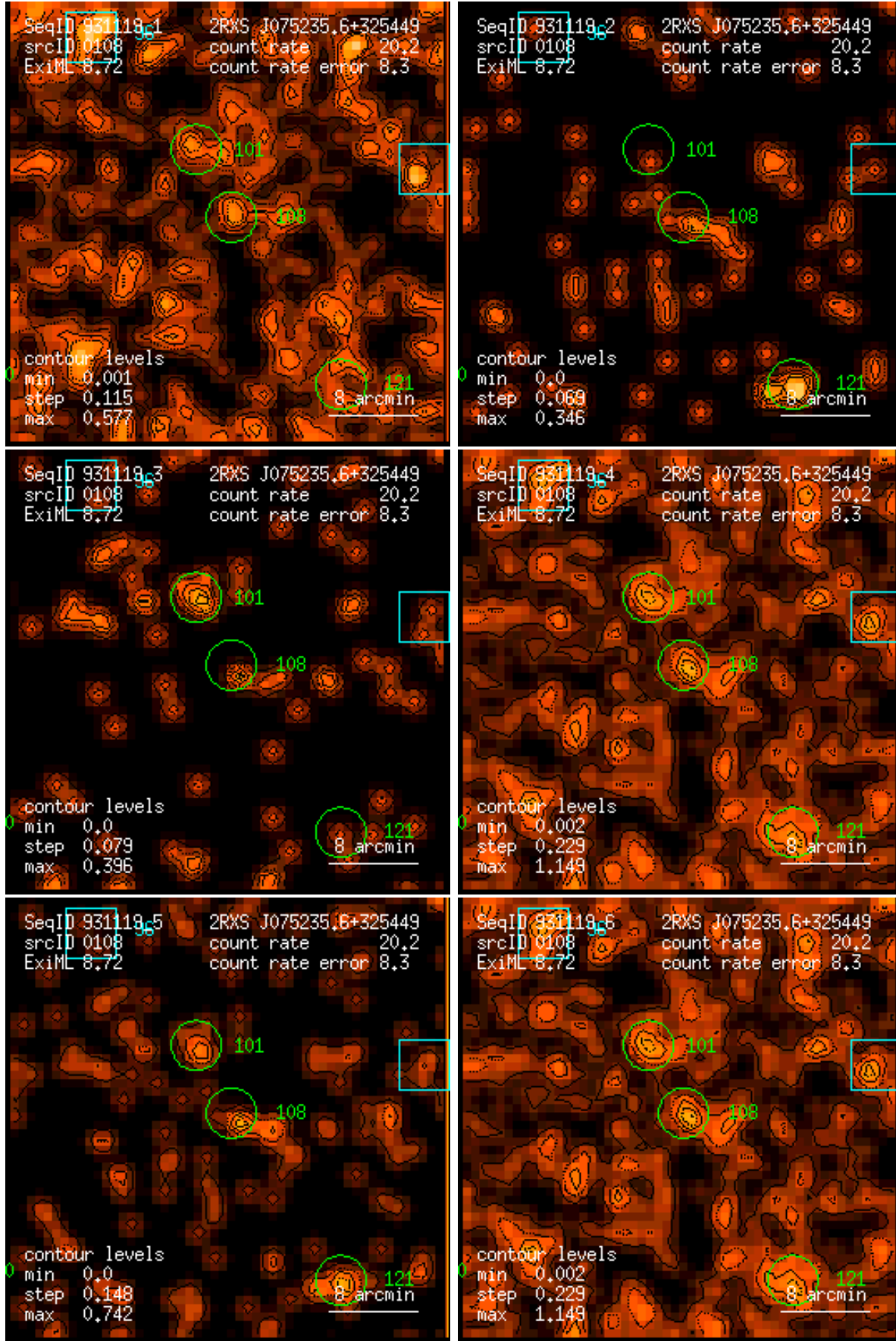
Figure 108: RASS 931119: detection 0108: band rate images, Gaussian filter: (1) PSPC channels 11 – 41, (2) 52 – 90, (3) 91 – 201, (4) 11 – 235, (5) 52 – 201, (6) 11 – 201. Broad band rates in counts/ks. Band rate contour levels in counts/ks/arcmin 2 .
