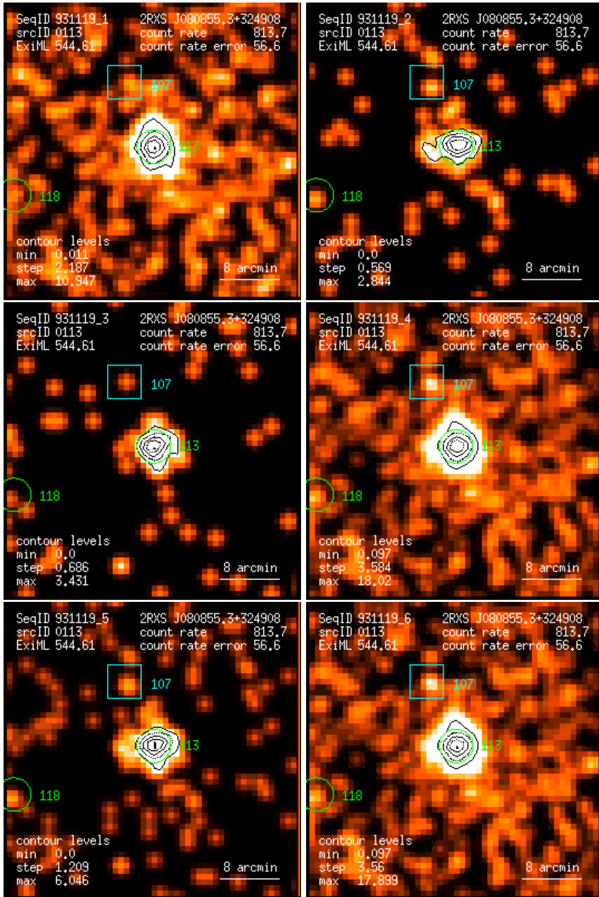
Figure 113: RASS 931119: detection 0113: band rate images, Gaussian filter: (1) PSPC channels 11 – 41, (2) 52 – 90, (3) 91 – 201, (4) 11 – 235, (5) 52 – 201, (6) 11 – 201. Broad band rates in counts/ks. Band rate contour levels in counts/ks/arcmin 2 .
