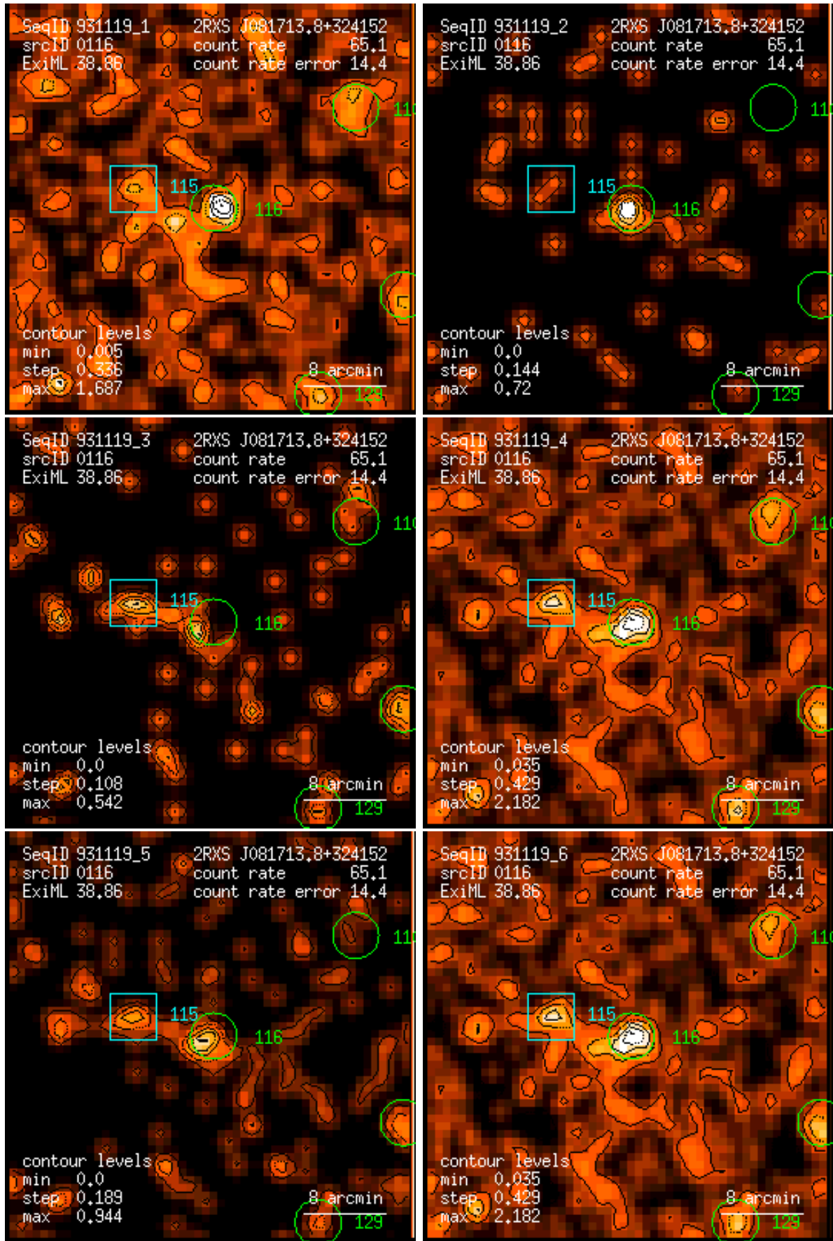
Figure 116: RASS 931119: detection 0116: band rate images, Gaussian filter: (1) PSPC channels 11 – 41, (2) 52 – 90, (3) 91 – 201, (4) 11 – 235, (5) 52 – 201, (6) 11 – 201. Broad band rates in counts/ks. Band rate contour levels in counts/ks/arcmin 2 .
