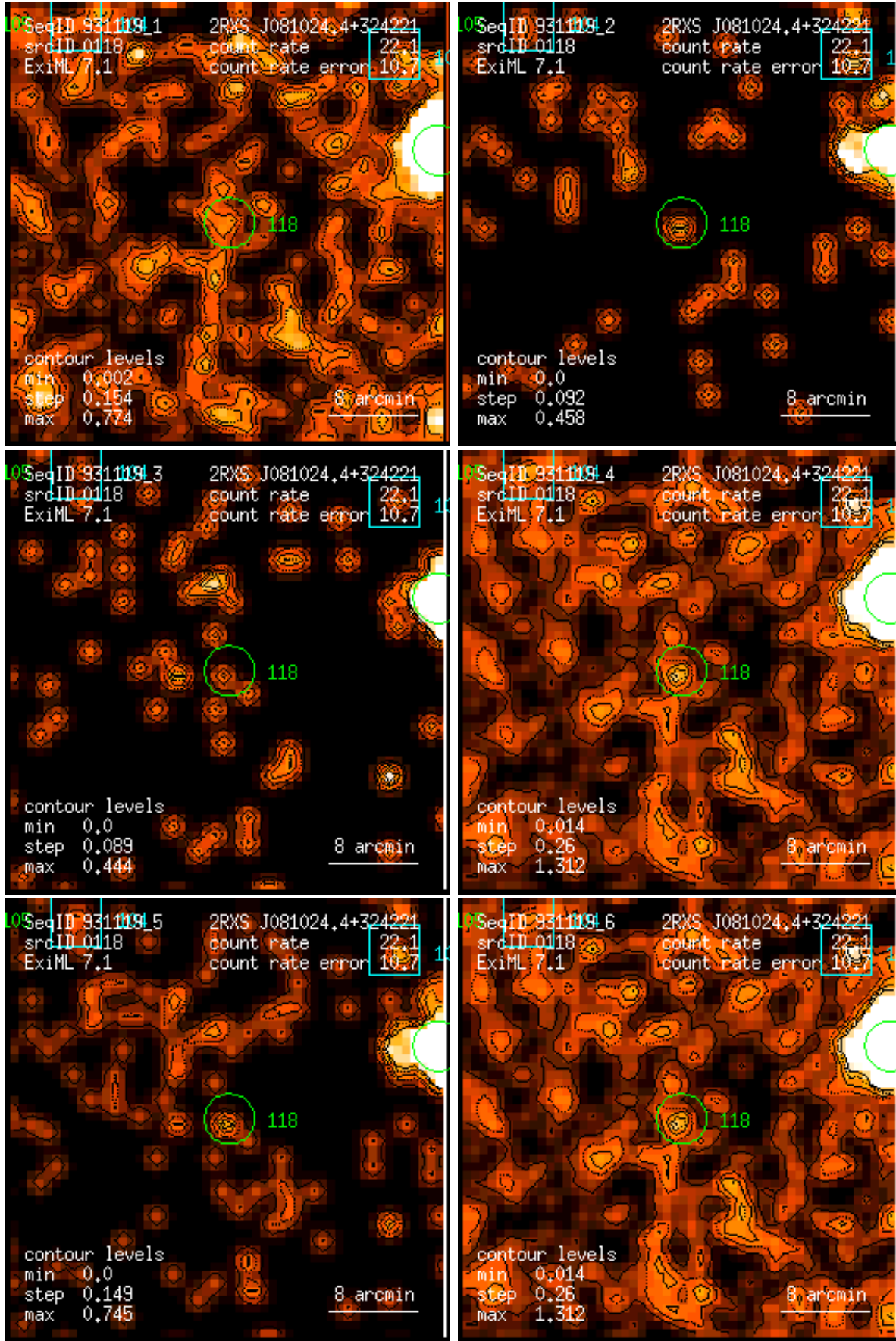
Figure 118: RASS 931119: detection 0118: band rate images, Gaussian filter: (1) PSPC channels 11 – 41, (2) 52 – 90, (3) 91 – 201, (4) 11 – 235, (5) 52 – 201, (6) 11 – 201. Broad band rates in counts/ks. Band rate contour levels in counts/ks/arcmin 2 .
